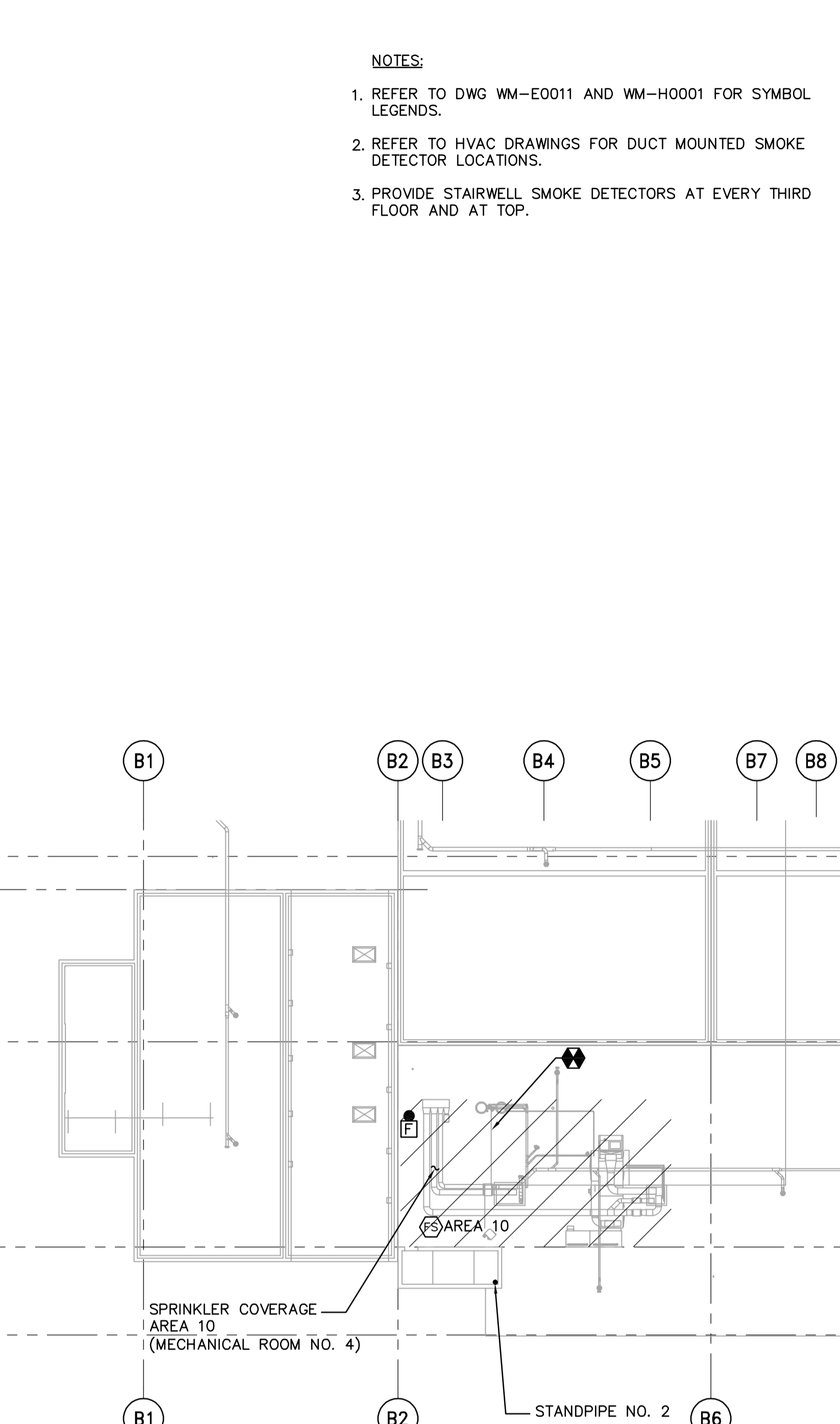
PARTIAL PLAN AT ELEVATION 251.450 1:300
