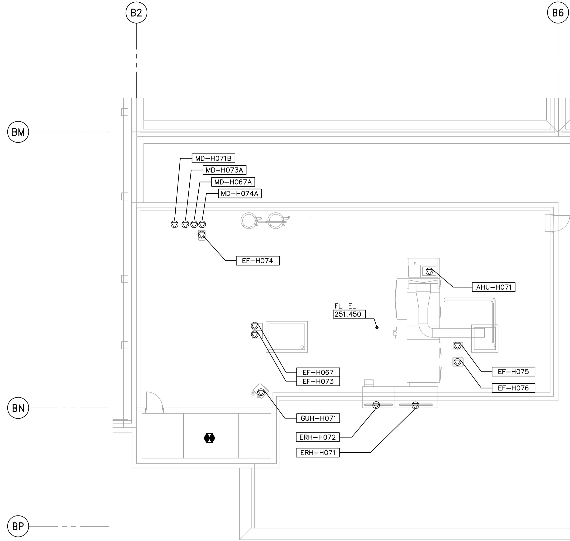
ROOF FACILITY PLAN 1:100
