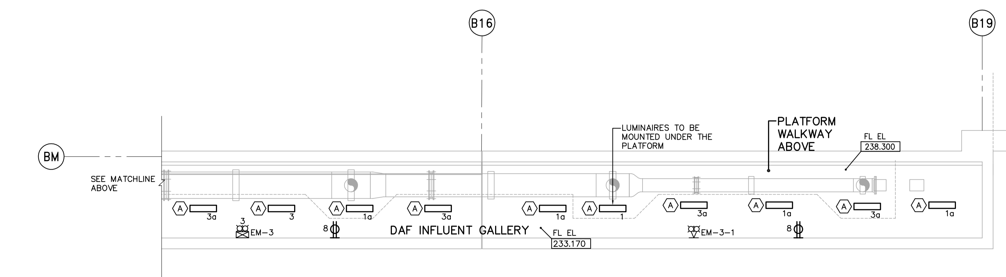
LOWER LEVEL POWER AND LIGHTING PLAN 1:100
