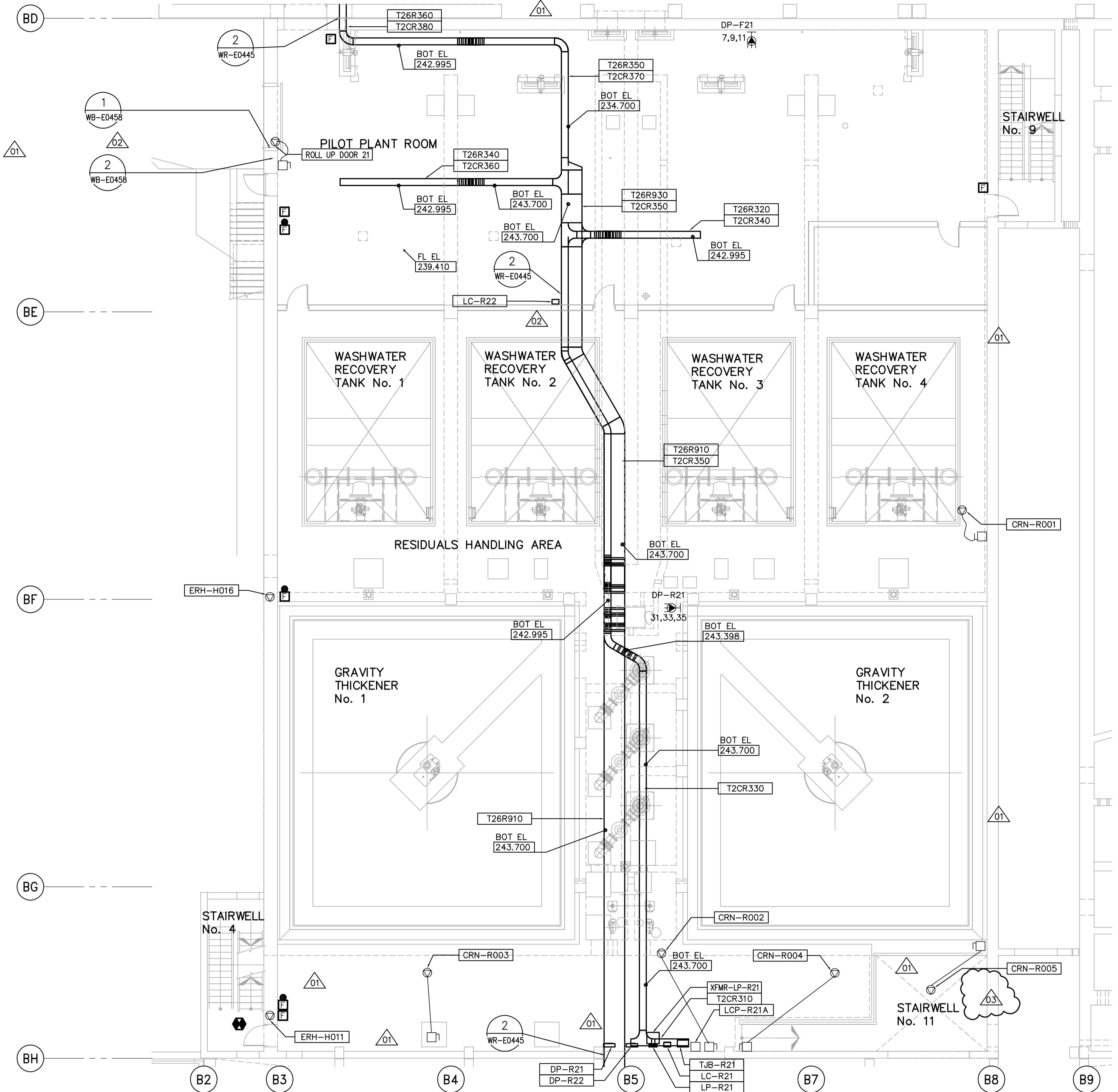
SECOND FLOOR FACILITY PLAN 1:100
