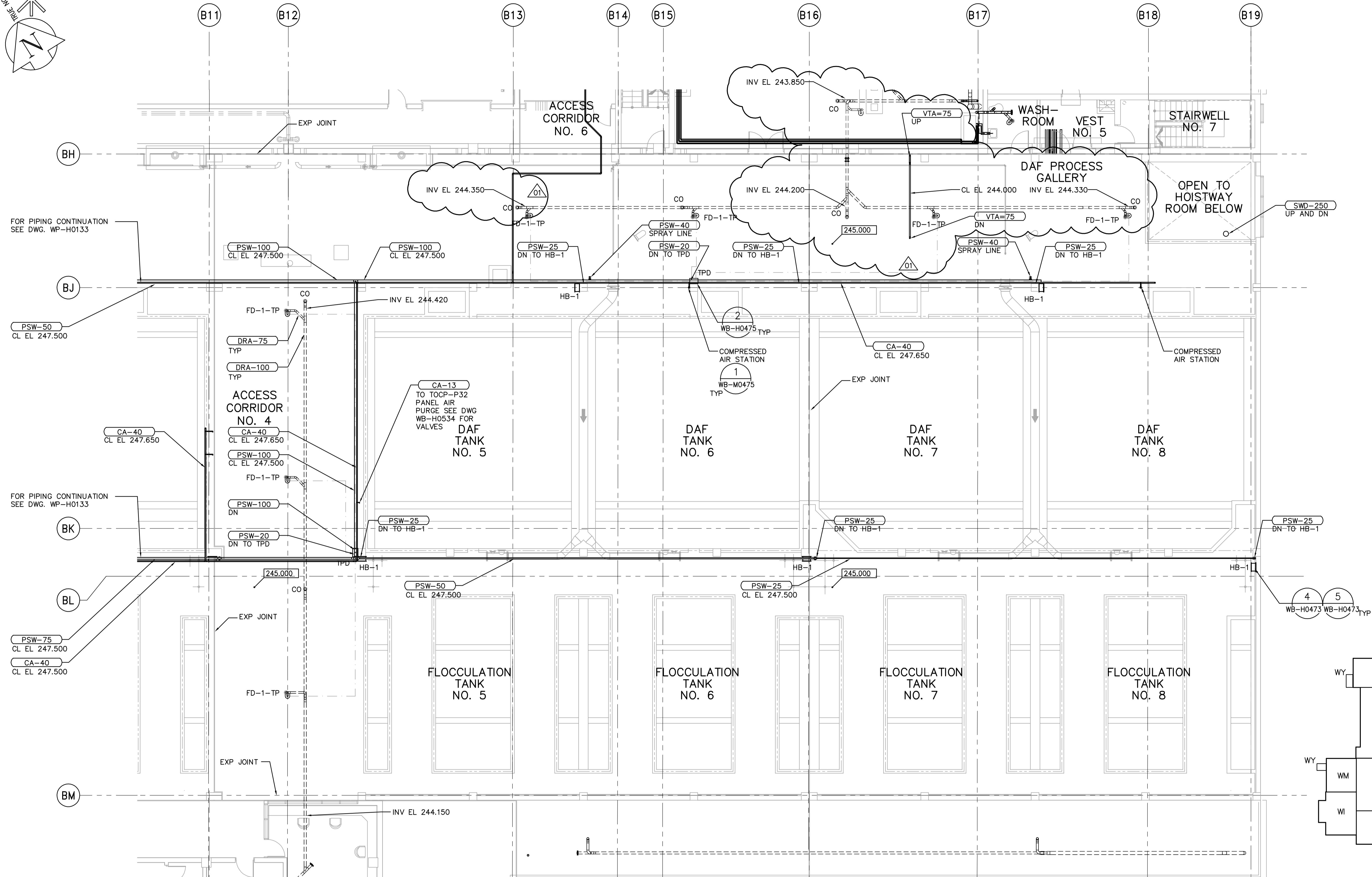
THIRD FLOOR PLAN 1:100
