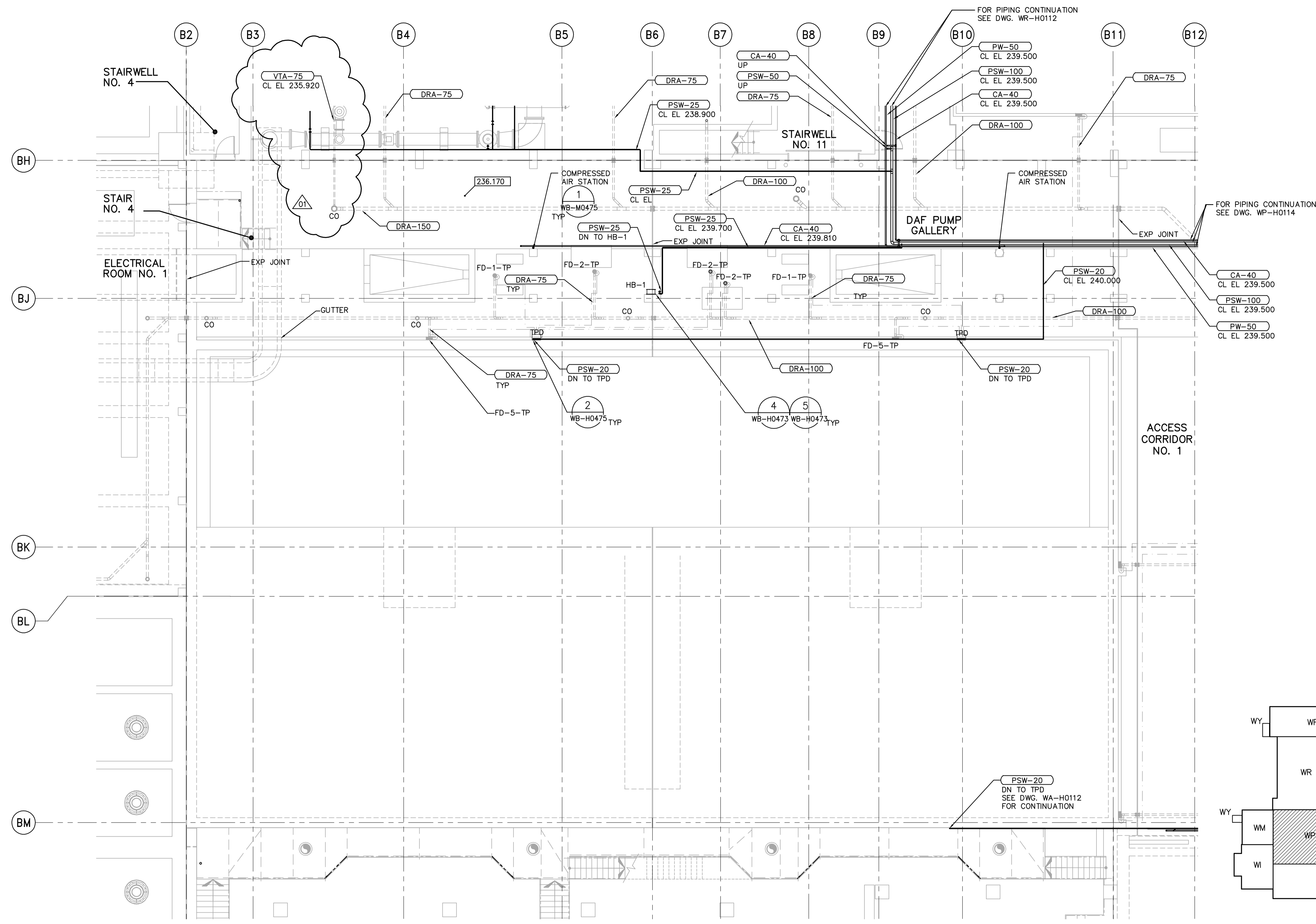
FIRST FLOOR PLAN 1:100
