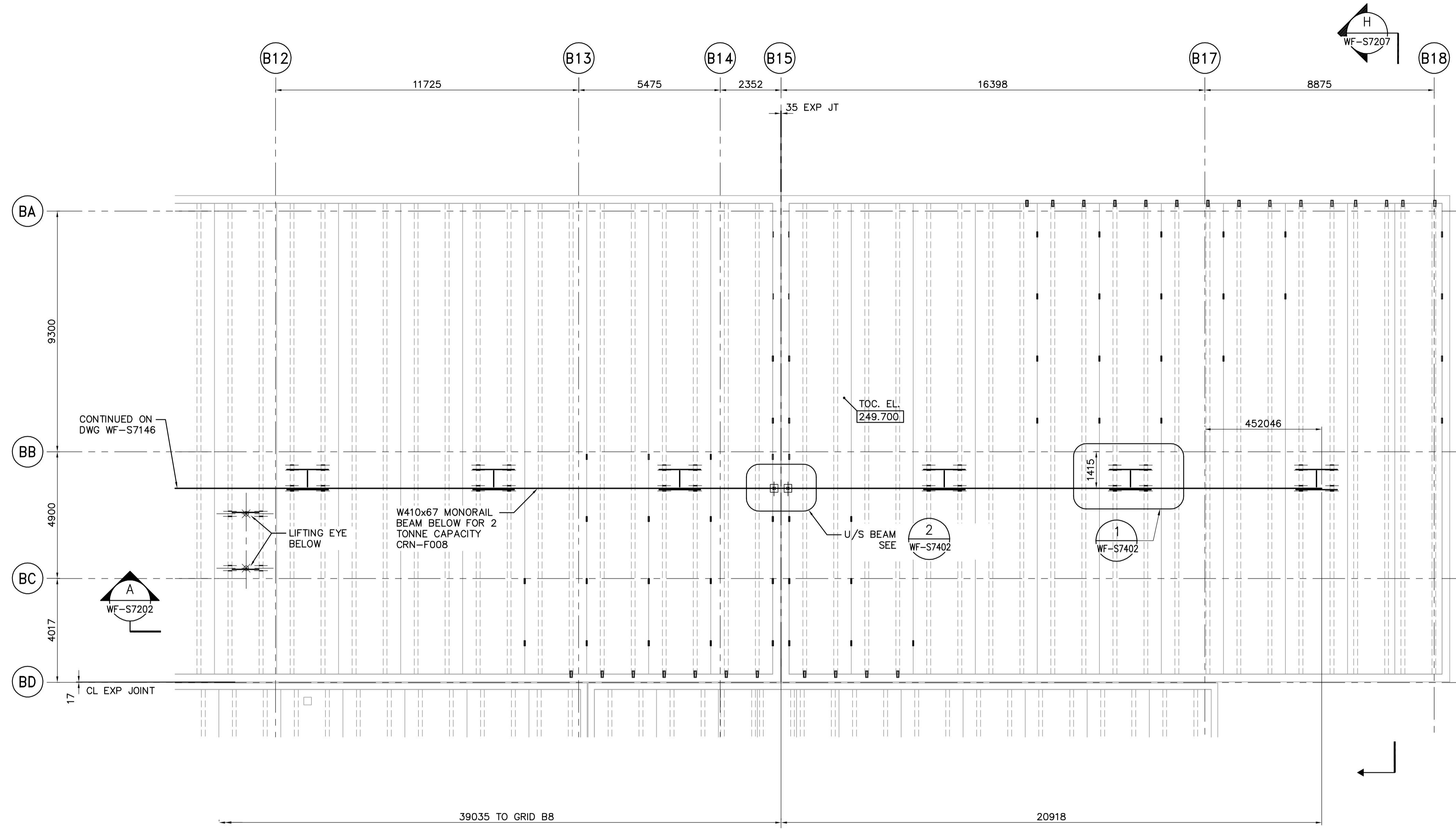
ROOF PLAN 1:100
