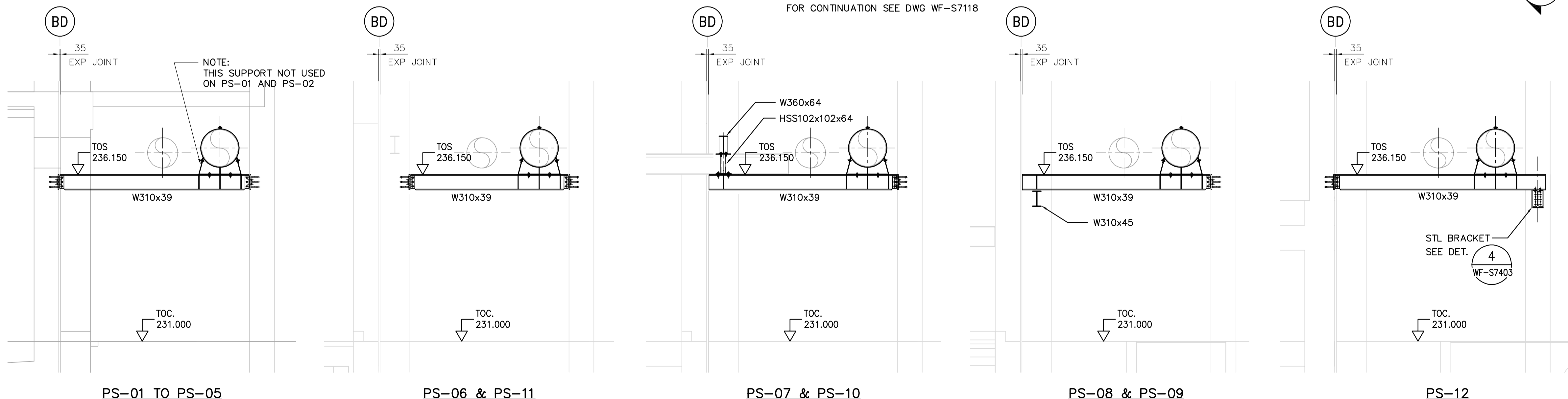
LOWER CHANNEL AT EL 238.500 1:100 NOTE: FOR CONTINUATION SEE DWG WF-S7118
