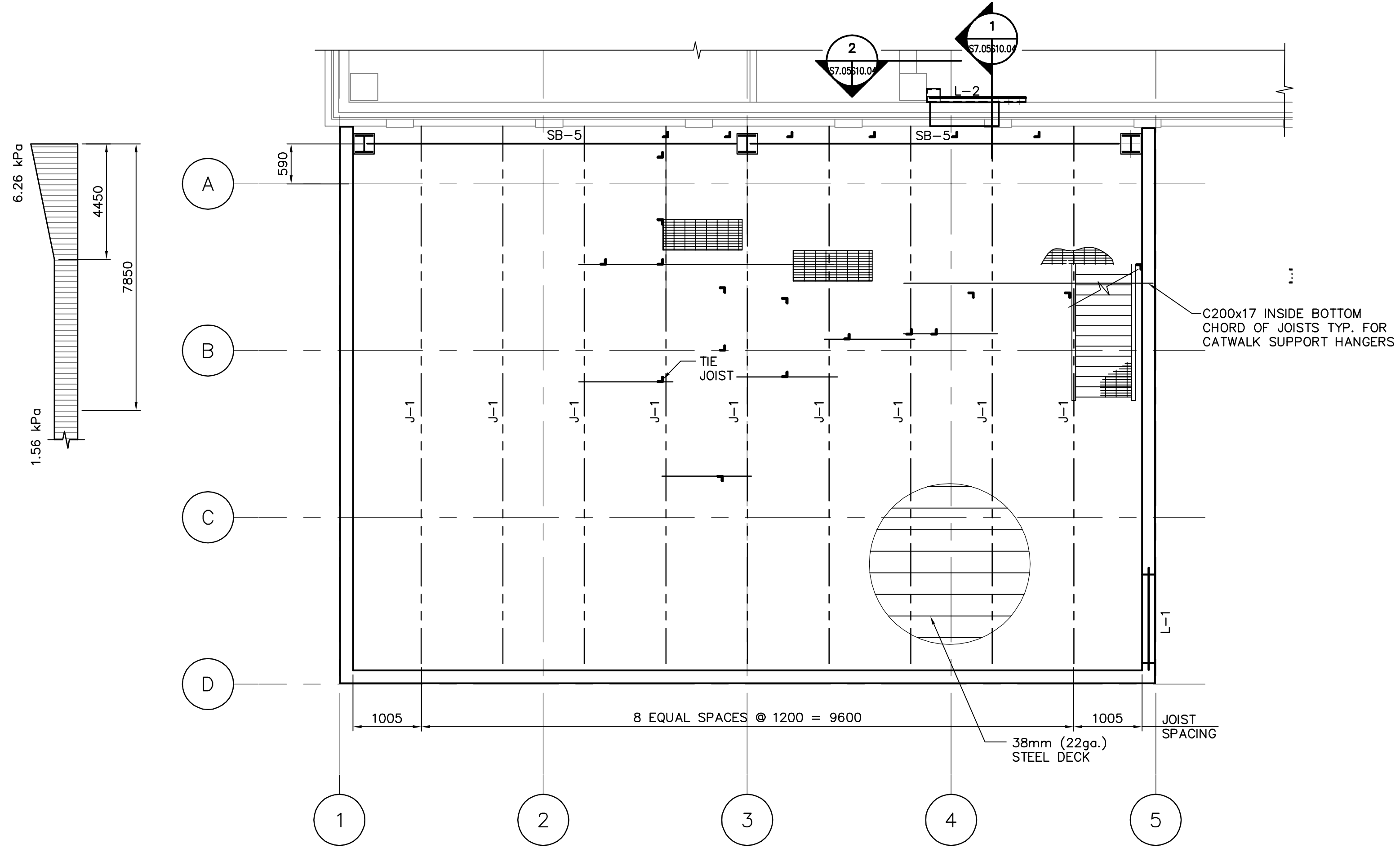
ROOF FRAMING PLAN SCALE : 1:50
