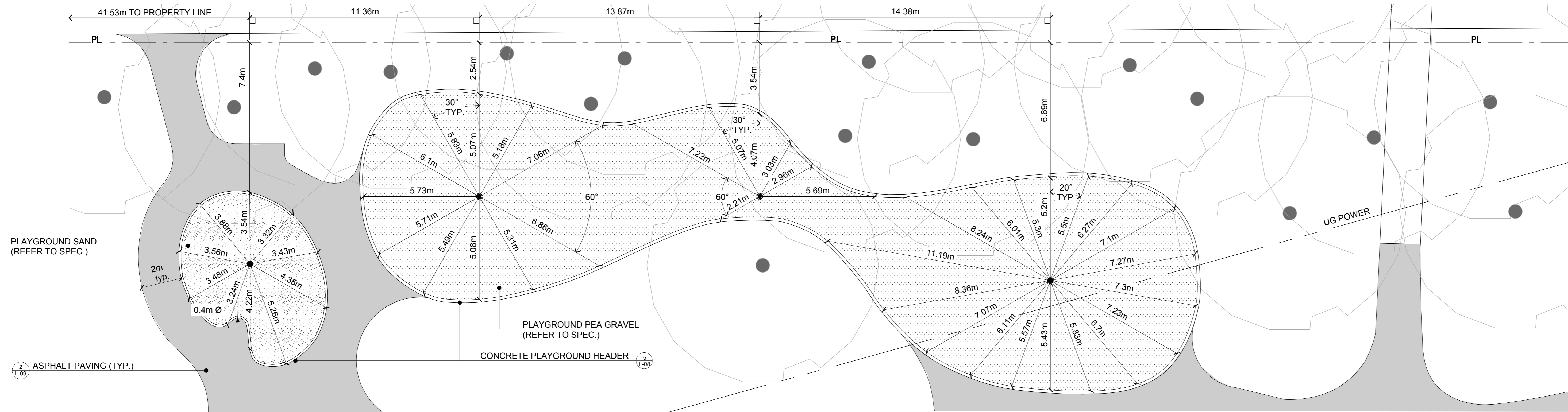
1 JUNIOR PLAY AREA PLAN SCALE: 1:100
