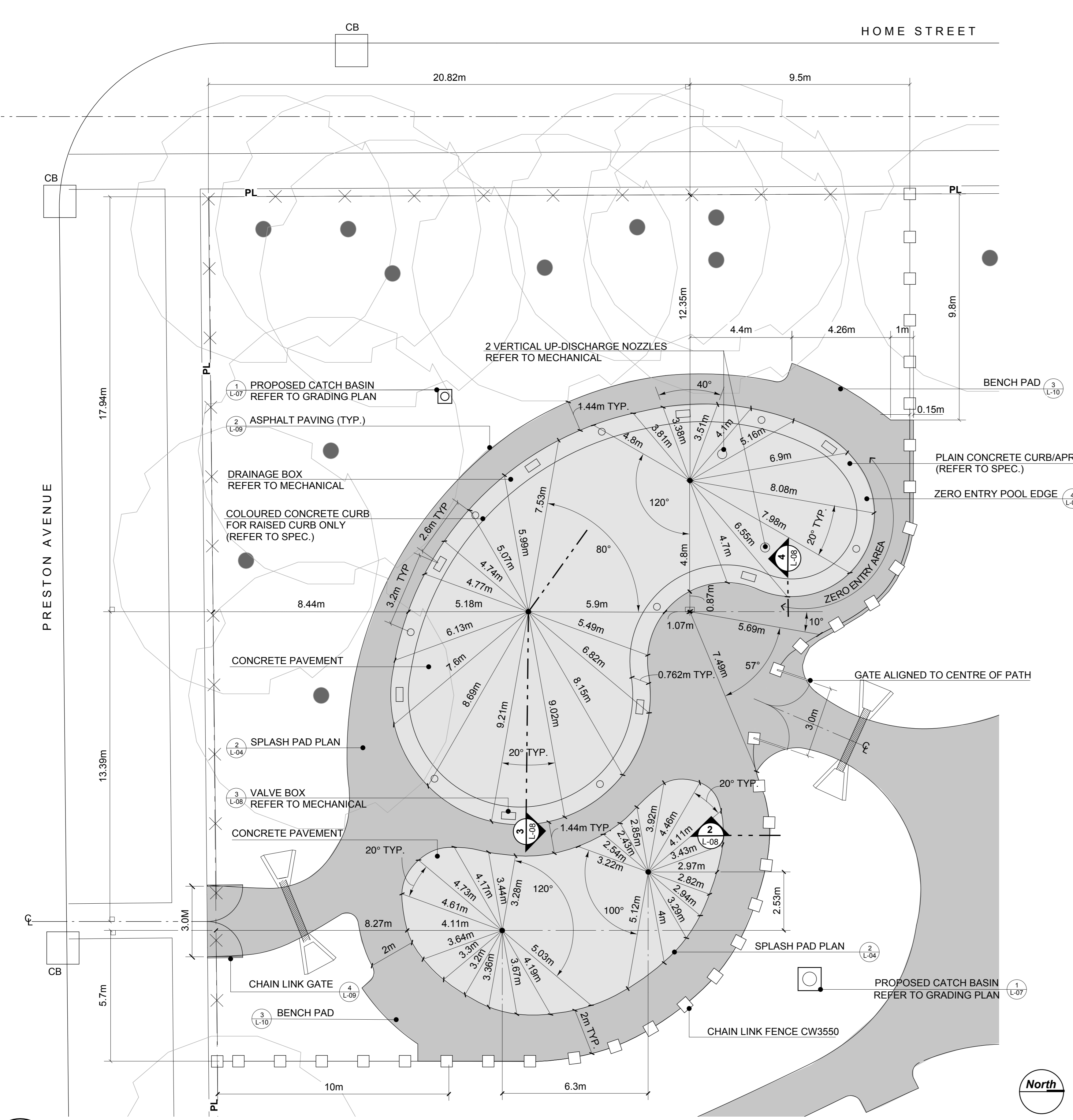
1 L-04 WATER PLAY AREA PLAN SCALE: 1:100
