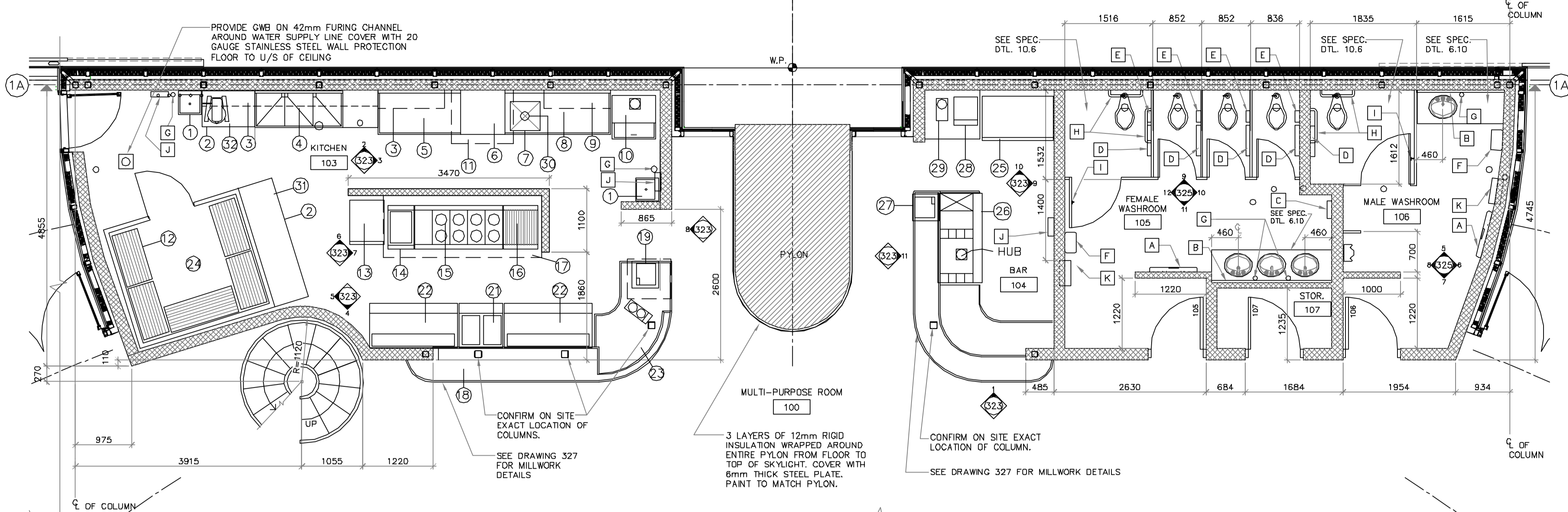
1 ENLARGED KITCHEN AND WASHROOM FLOOR PLANS
