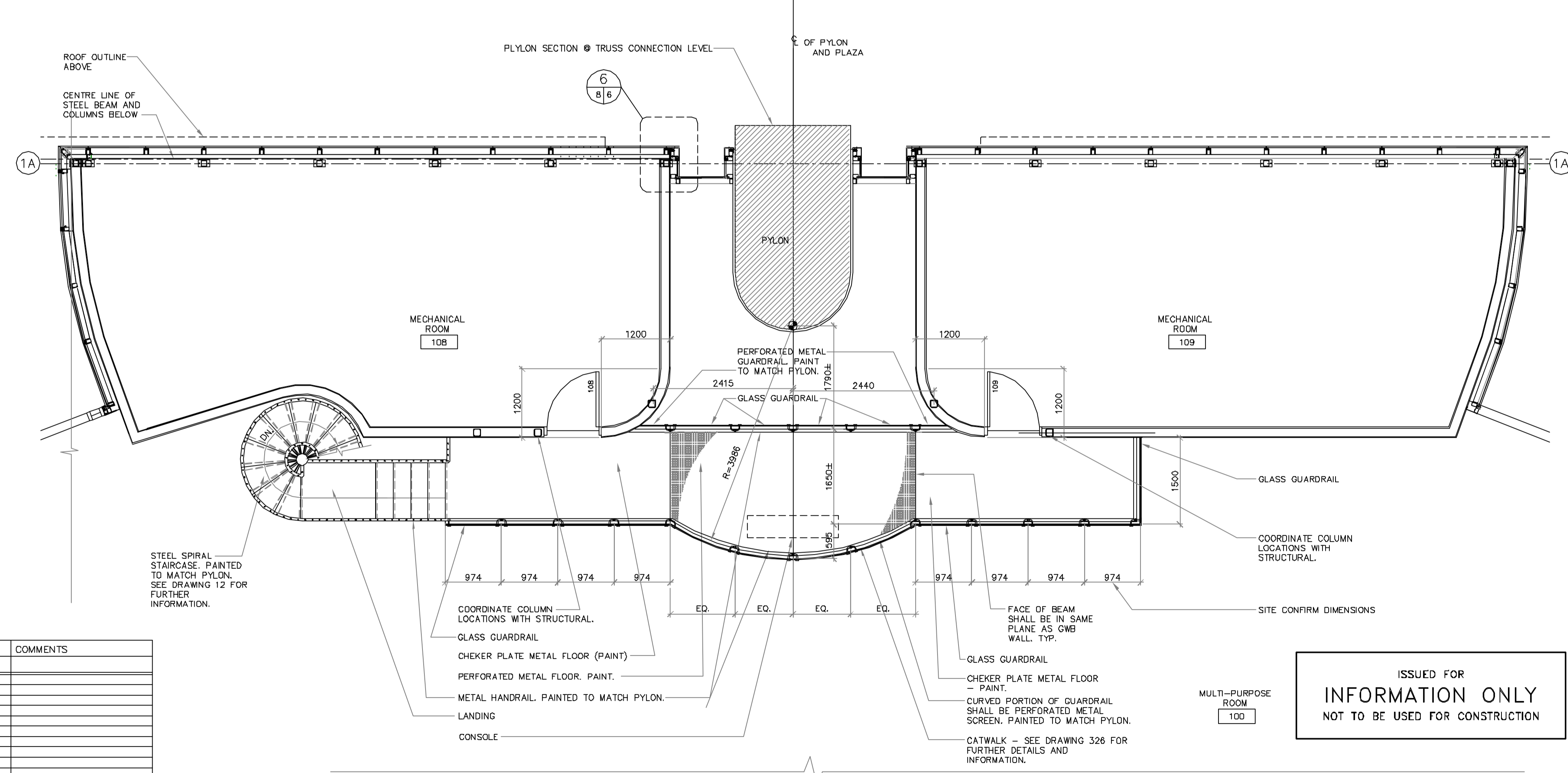
2 ENLARGED MECHANICAL ROOM FLOOR PLANS
