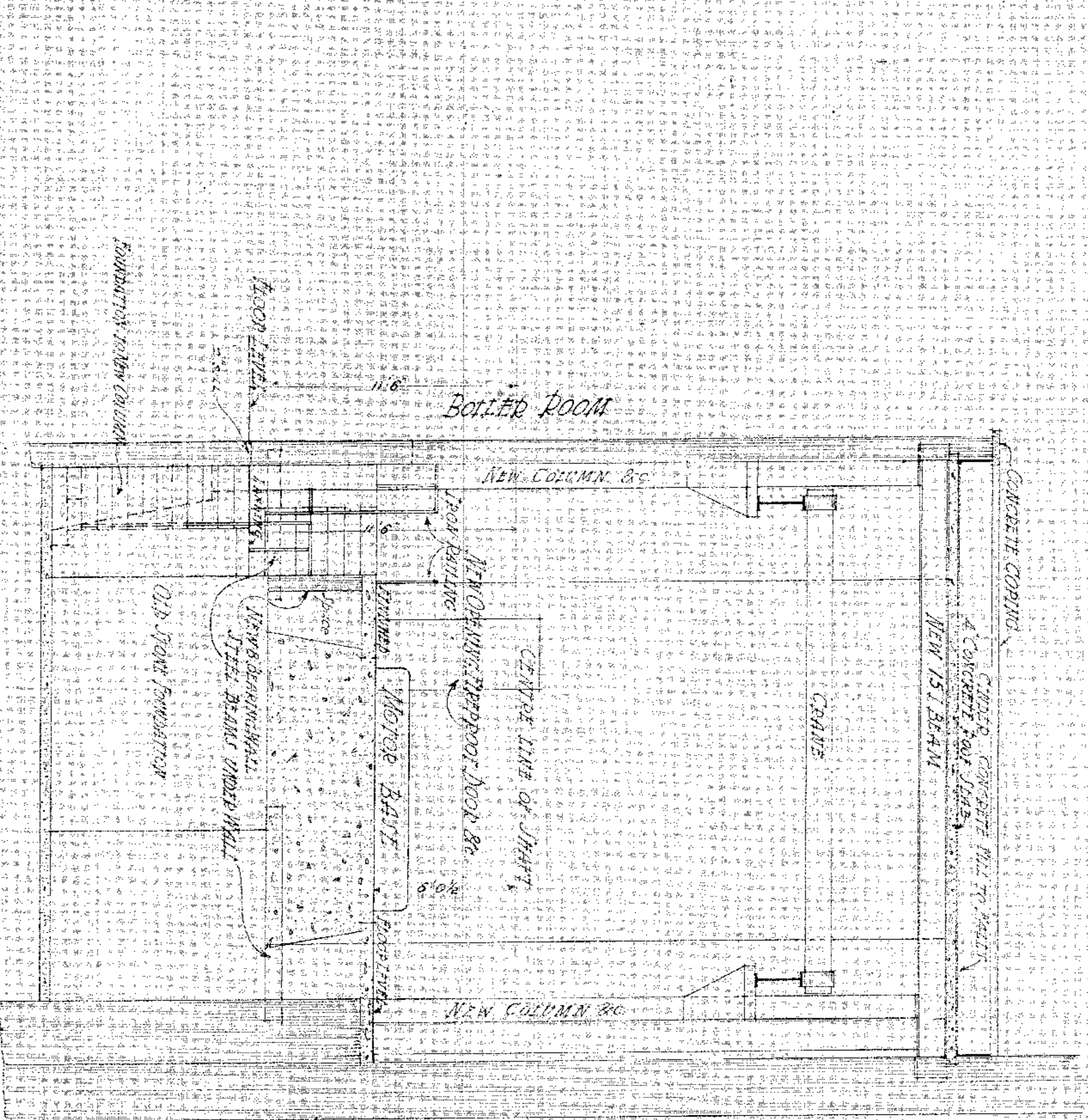
SECTION ON LINE CC
