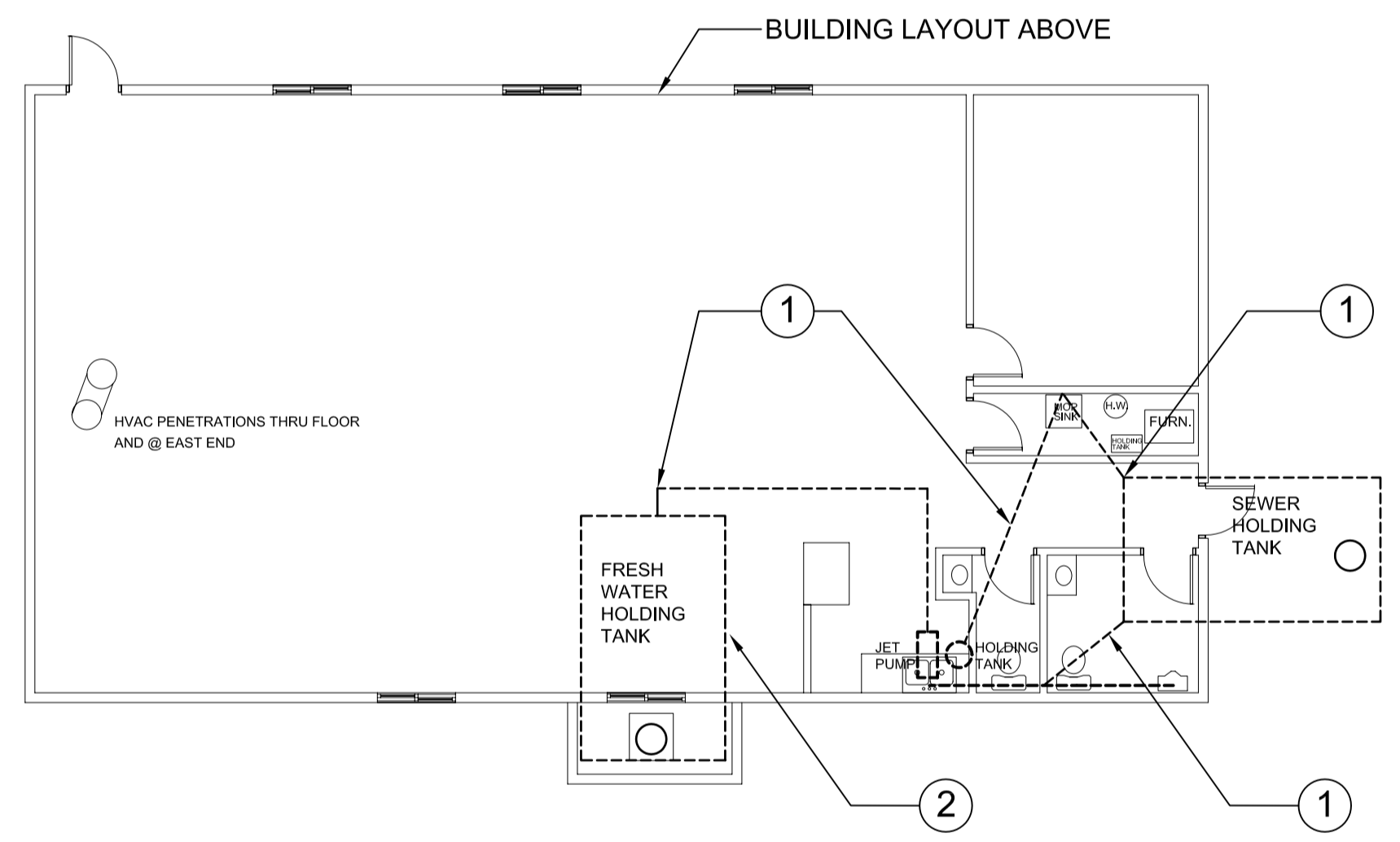
PLAN -NEW PLUMBING & HVAC RECONNECTIONS SCALE: 1/8" = 1'-0"
