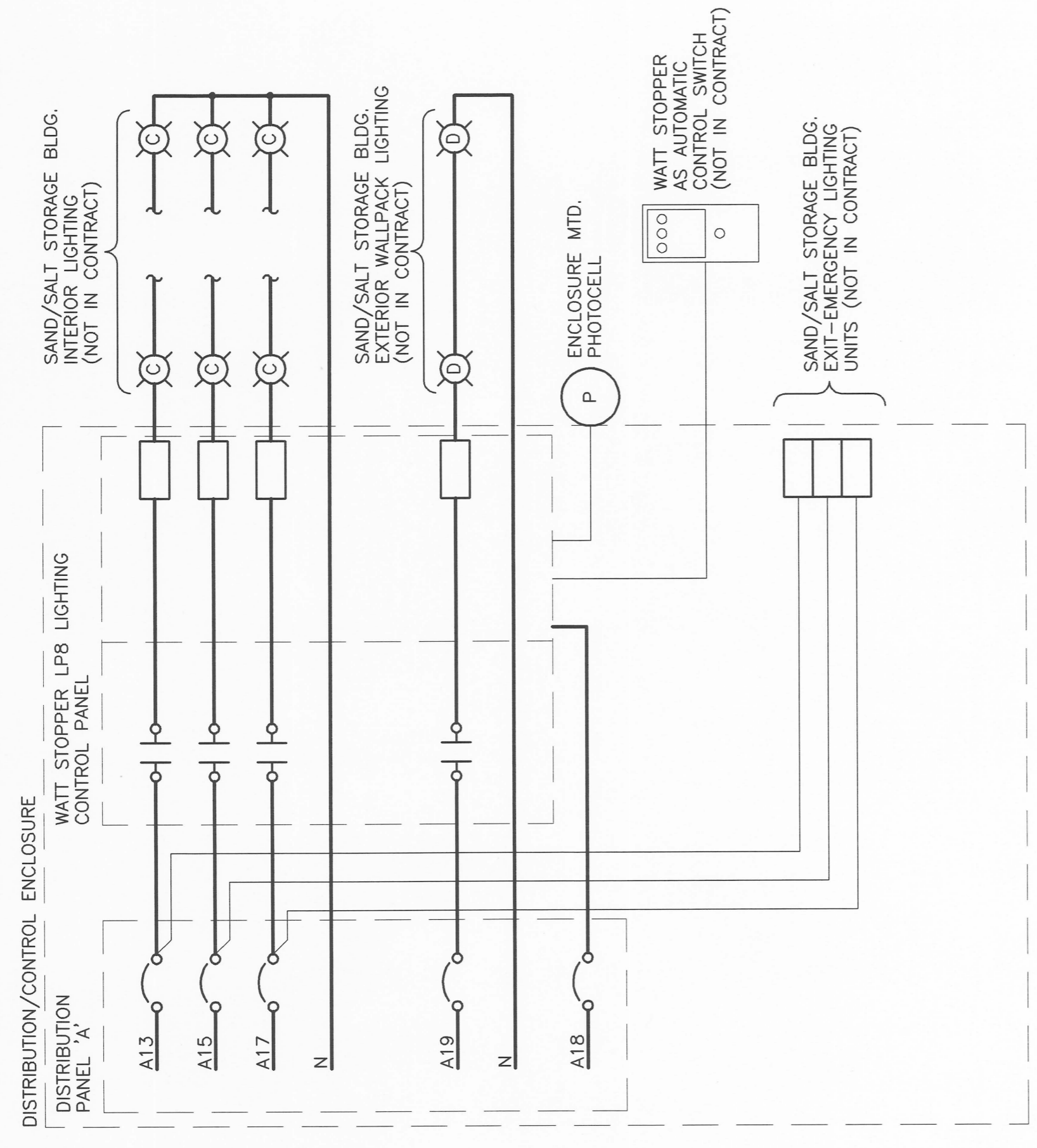
B LIGHTING CONTROL SCHEMATIC N.T.S.
