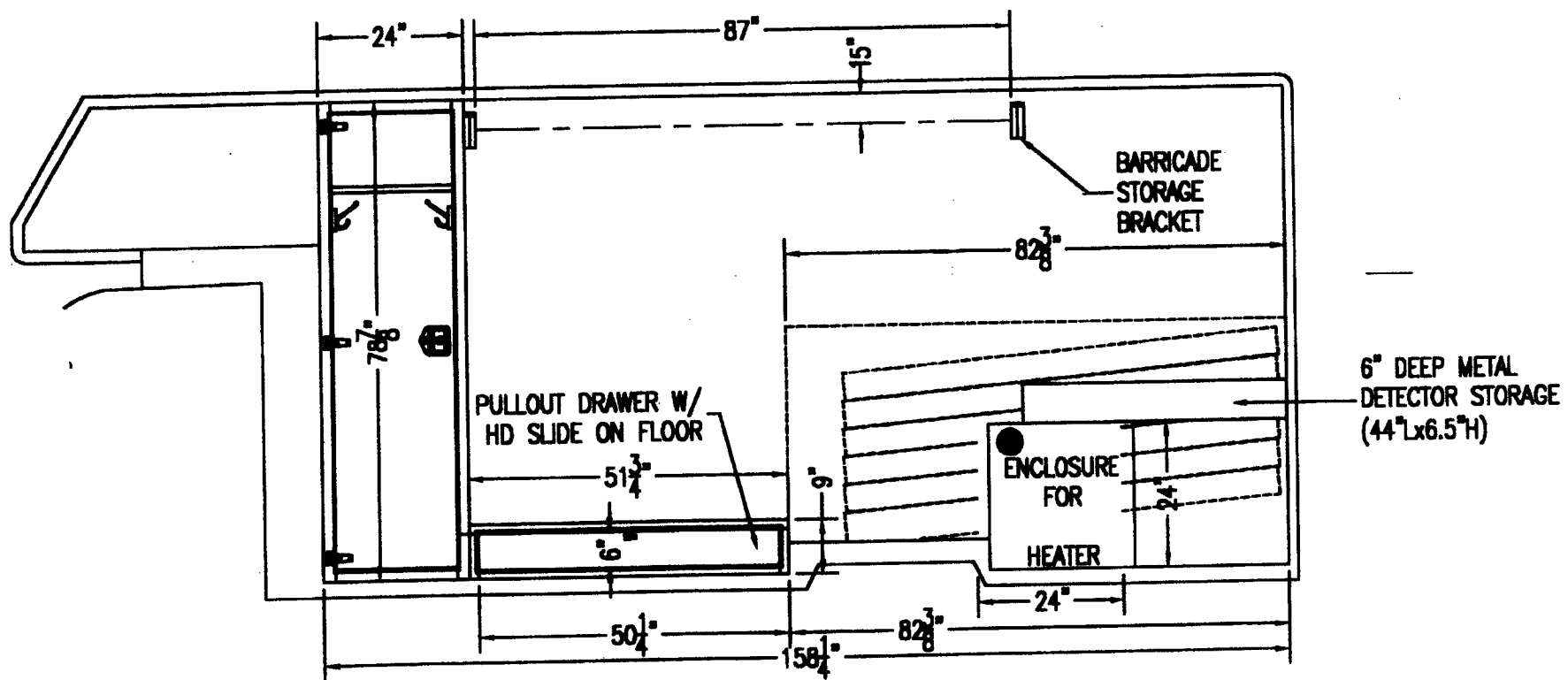
CURBSIDE INTERIOR
