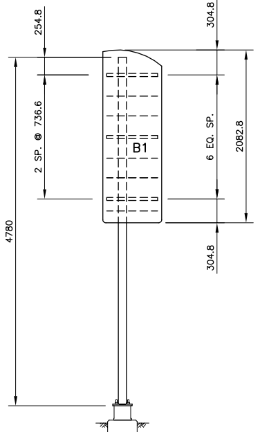
POST P2-R, SIGN B1
