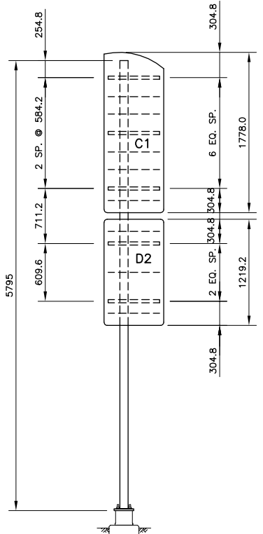
POST P8-R, SIGNS C1+D2
