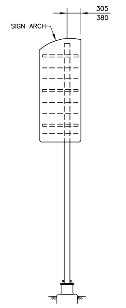
LHS (LEFT HAND SIDE) MOUNTED SIGN
