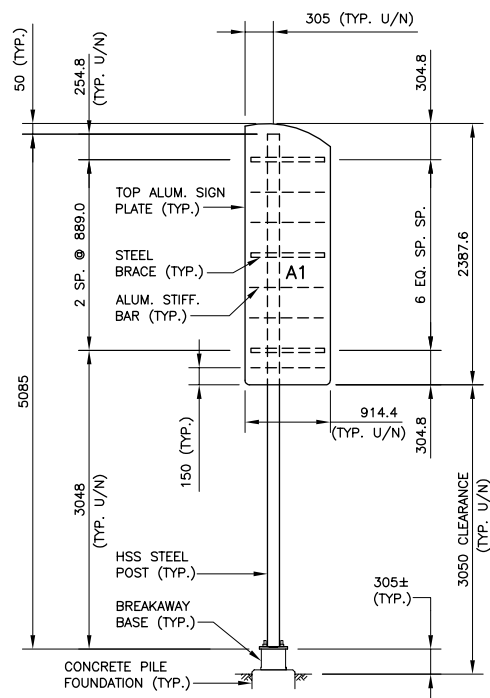
POST P1-R, SIGN A1 R=RHS (RIGHT HAND SIDE) MOUNTED SIGNS
