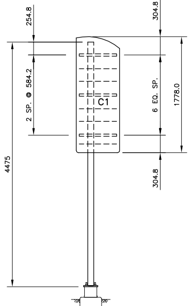
POST P3-R, SIGN C1
