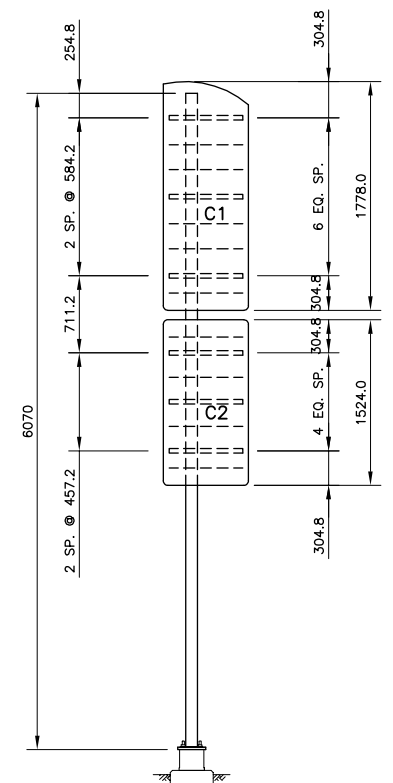
POST P7-R, SIGNS C1+C2
