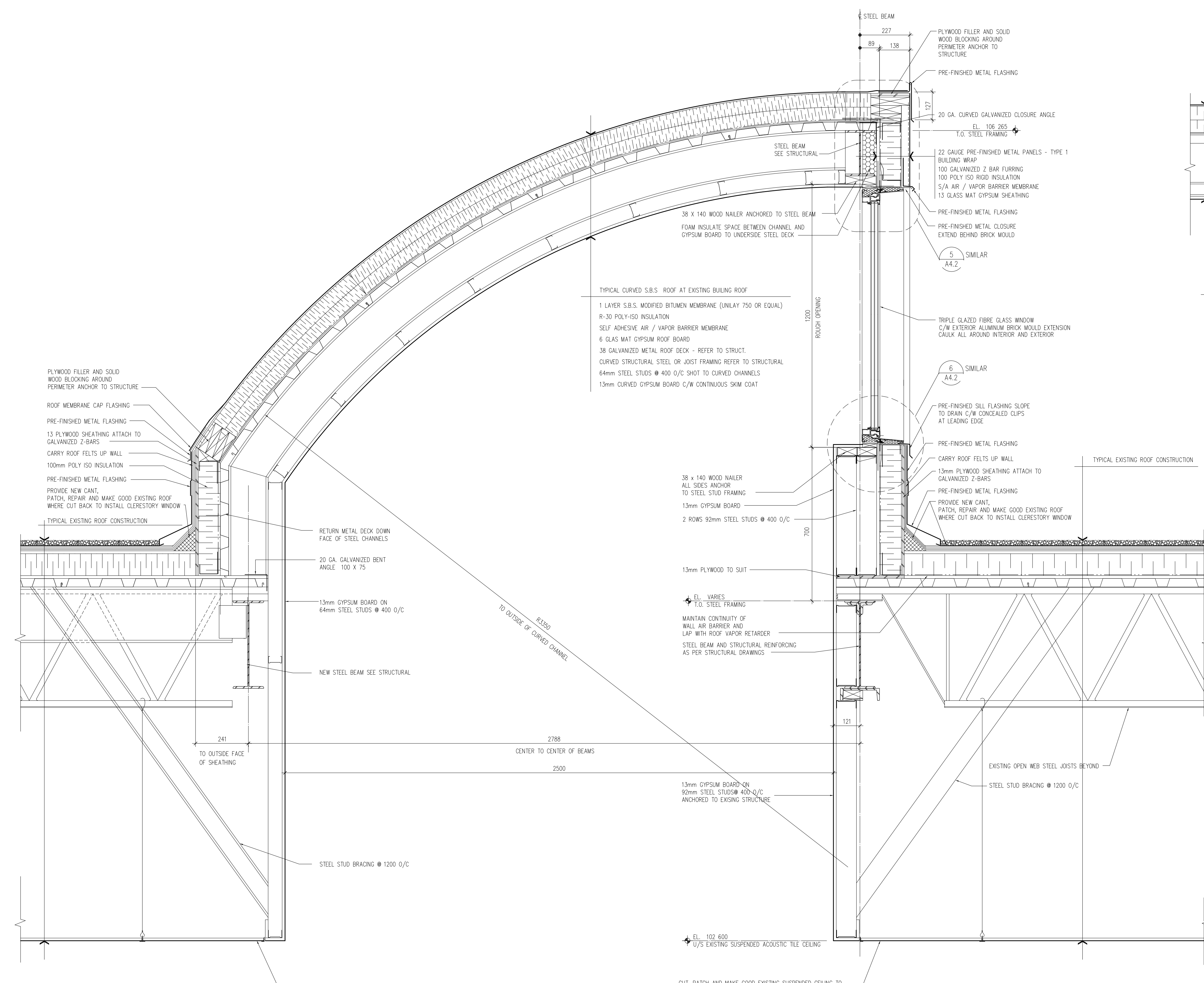
A6.7 2 CROSS SECTION A CURVED CLERESTORY (TYPICAL) SCALE: 1:10
