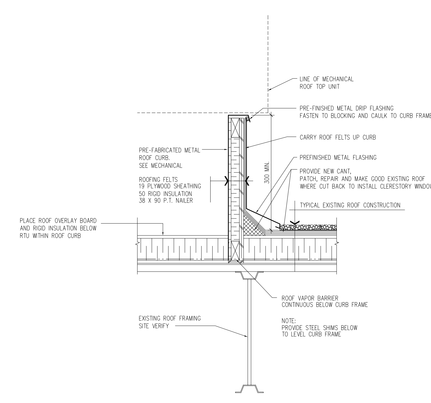
A6.7 4 CURB DETAIL AT NEW ROOF TOP UNITS ON EXISTING ROOF SCALE: 1:10
