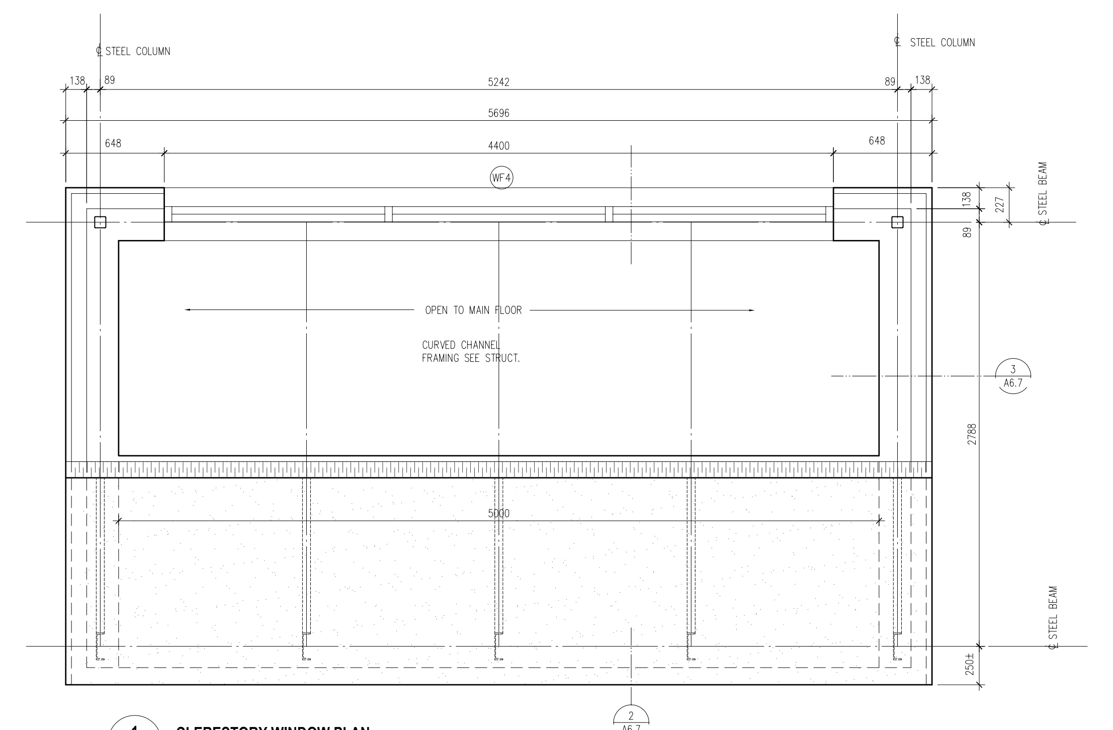
A6.7 1 CLERESTORY WINDOW PLAN 1:20
