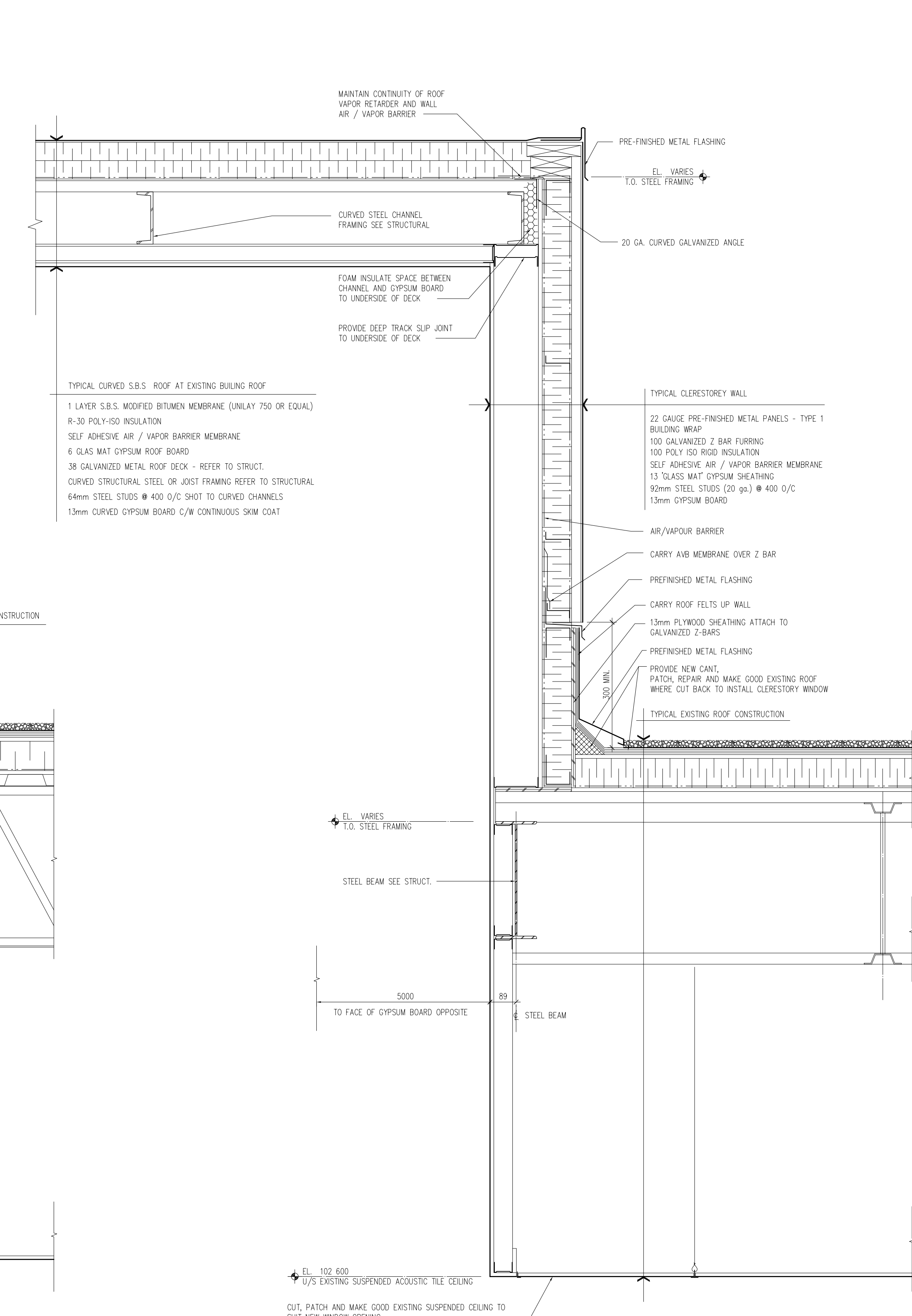
A6.7 2.10 CROSS SECTION AT CURVED CLERESTORY WINDOW (TYPICAL) SCALE: 1:10
