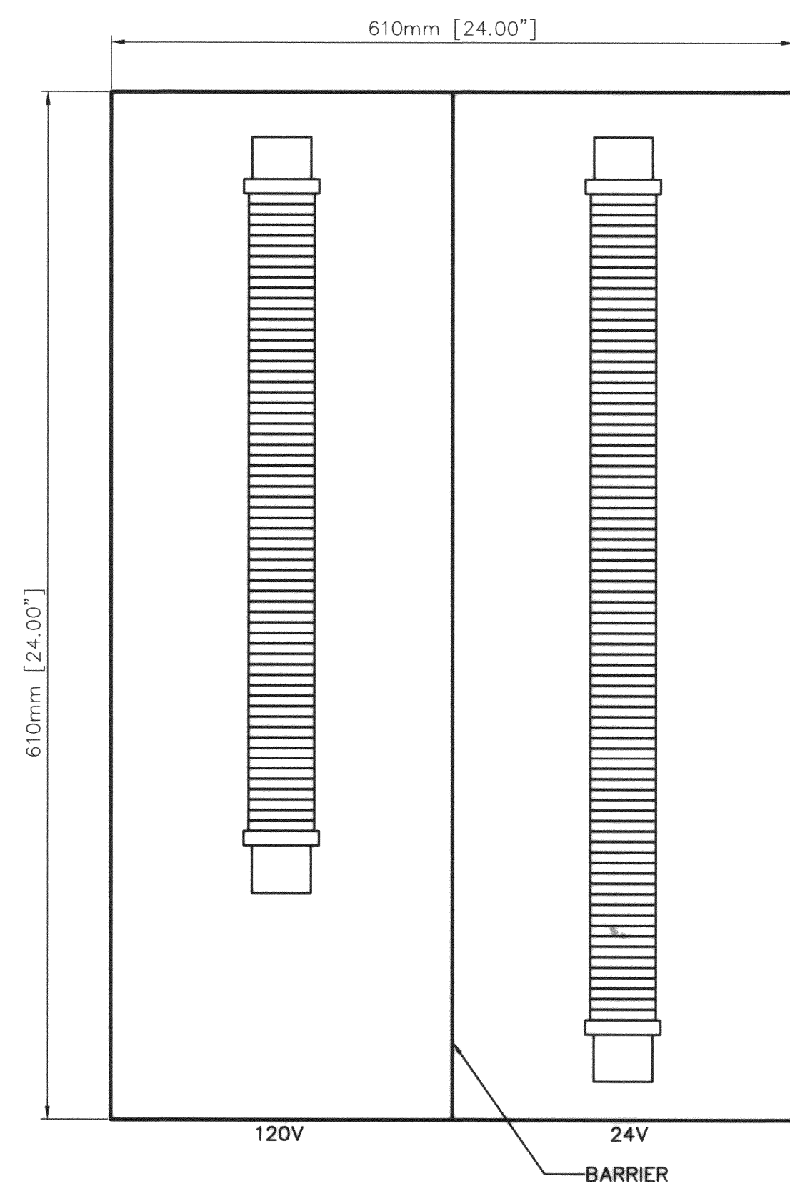
TYPICAL TERMINAL CABINET LAYOUT FRONT INTERIOR ELEVATION
