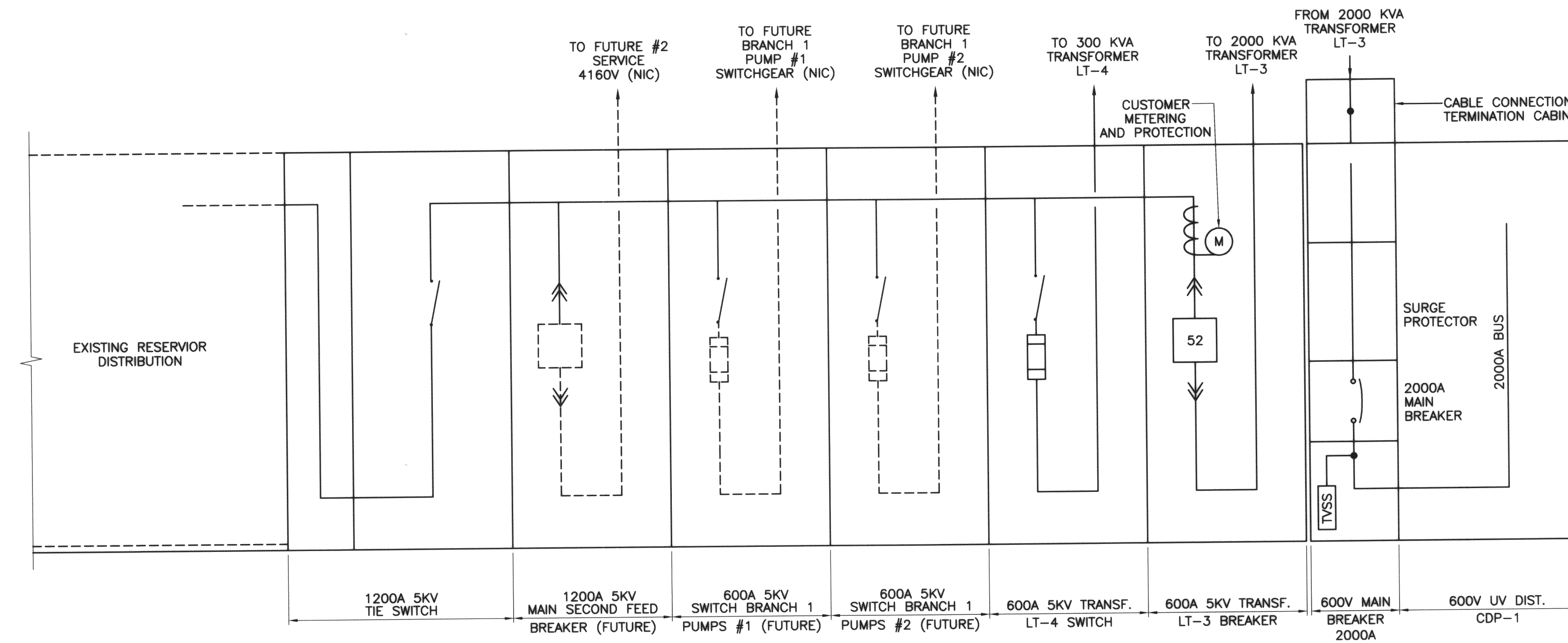
UV DISTRIBUTION FRONT ELEVATION SCALE: 1:20
