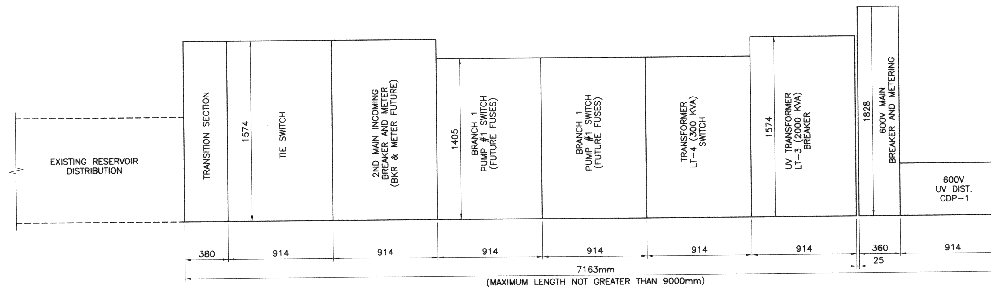
UV DISTRIBUTION PLAN SCALE: 1:20
