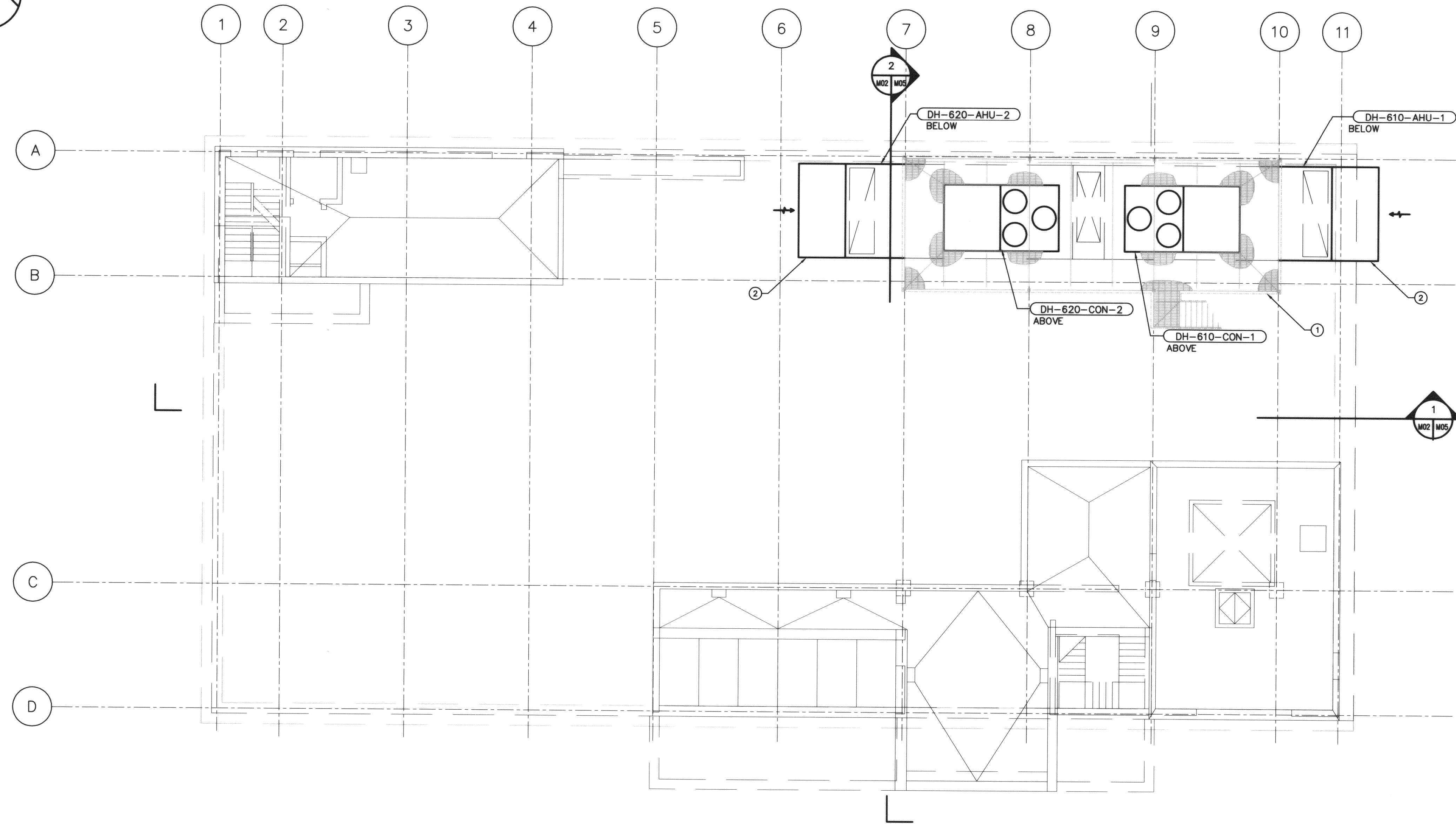
MECHANICAL ROOF PLAN ABOVE EL. 236.500m SCALE: 1:100
