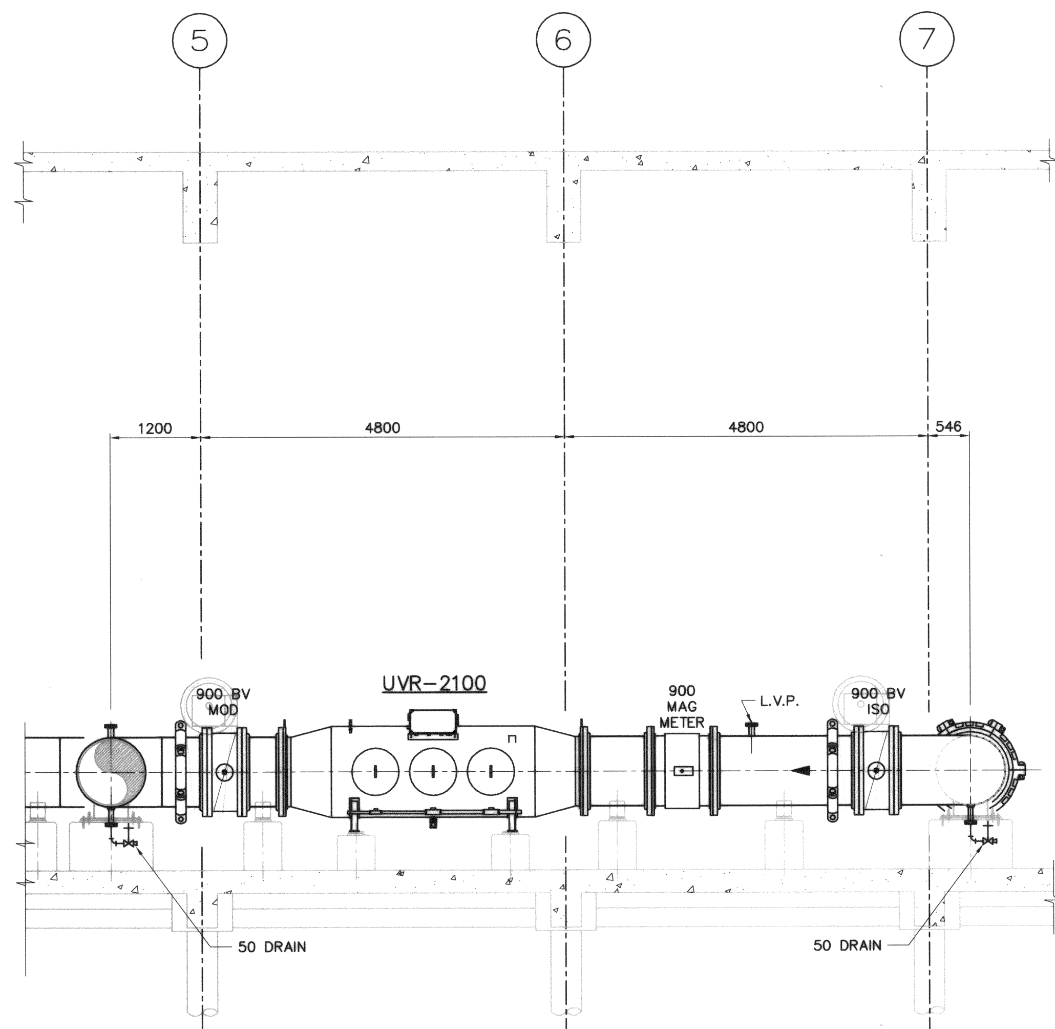
H SECTION P21 SCALE 1:50
