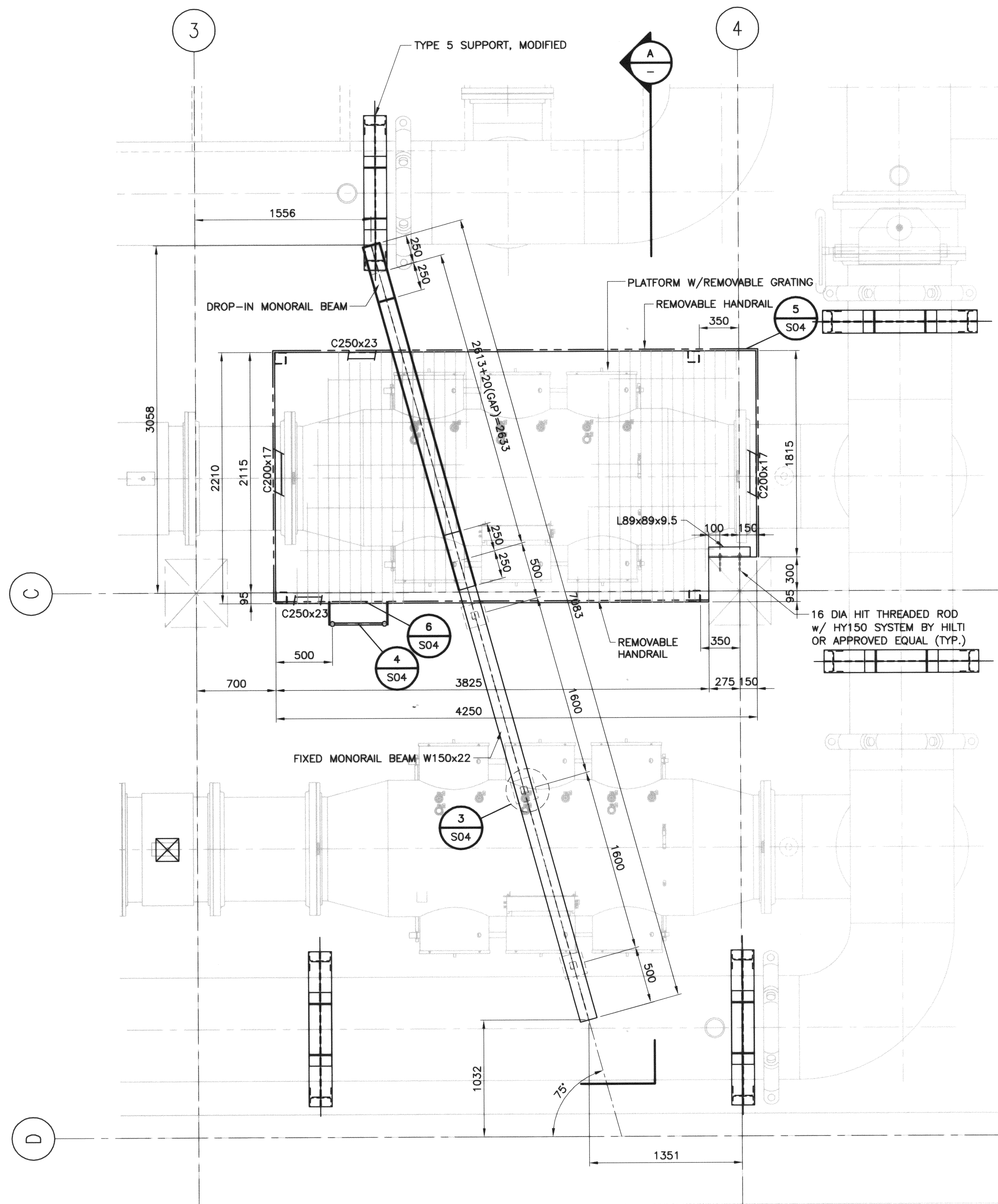
6 MONORAIL BEAM AND PLATFORM PLAN S01 SCALE 1:25
