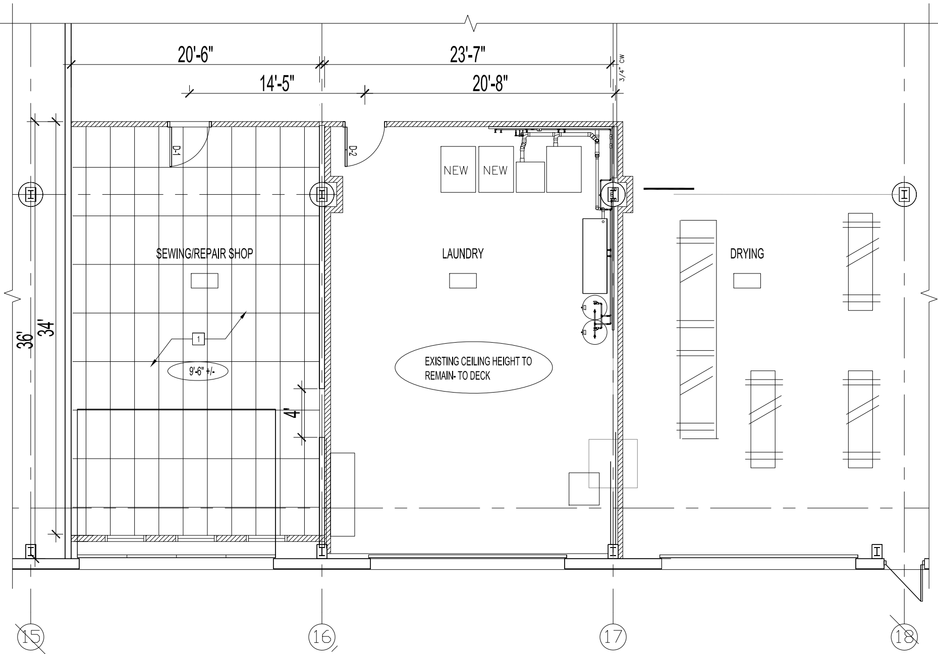
PARTIAL MAIN FLOOR PLAN - REFLECTED CEILING PLAN SCALE: 1/4" = 1'-0"
