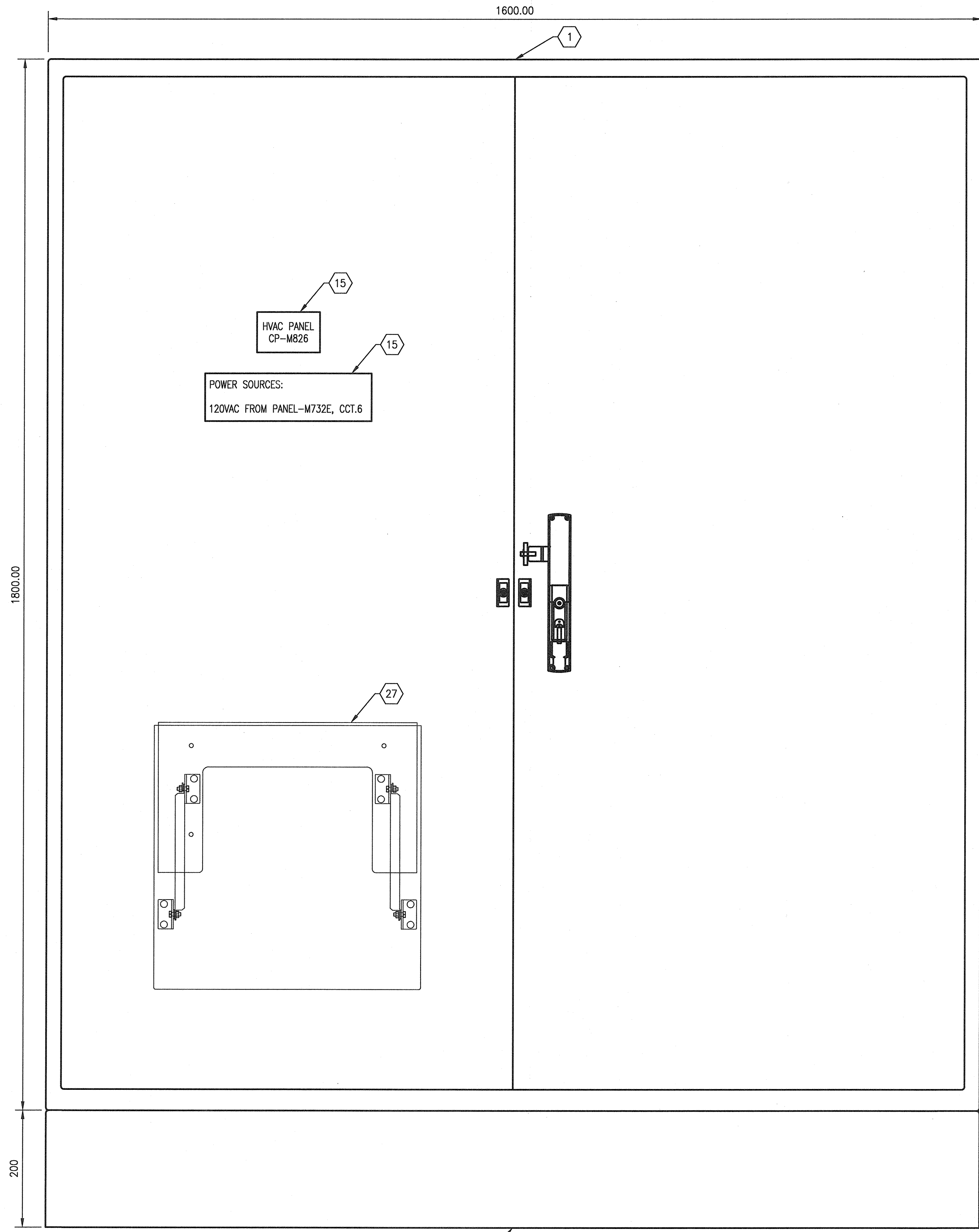
EXTERIOR PANEL VIEW SCALE: 1 : 5
