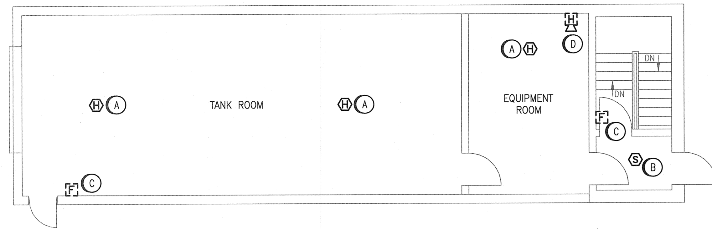
CHLORINE BUILDING GROUND LEVEL - FIRE ALARM SCALE: 1 : 50
