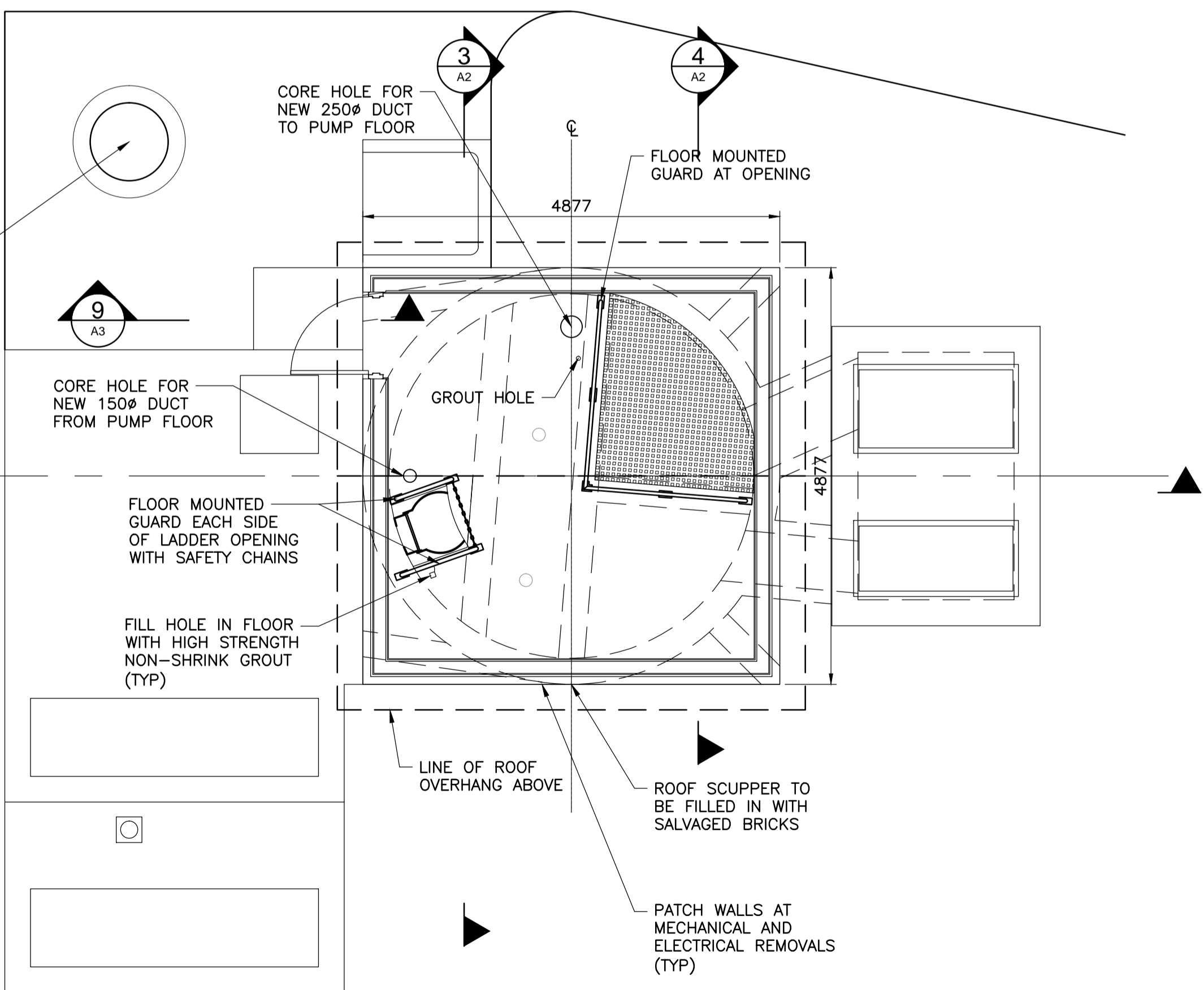
PLAN AT MOTOR FLOOR 1:50
