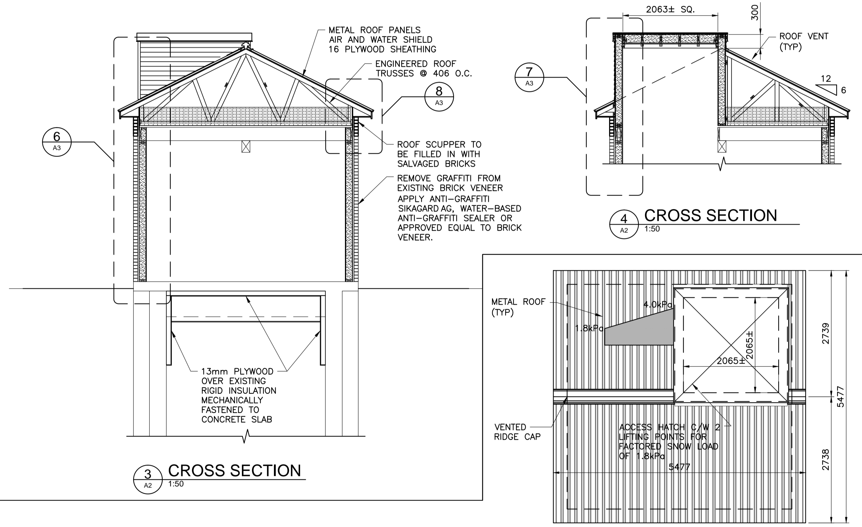
ROOF PLAN WITH SNOW LOADINGS 1:50
