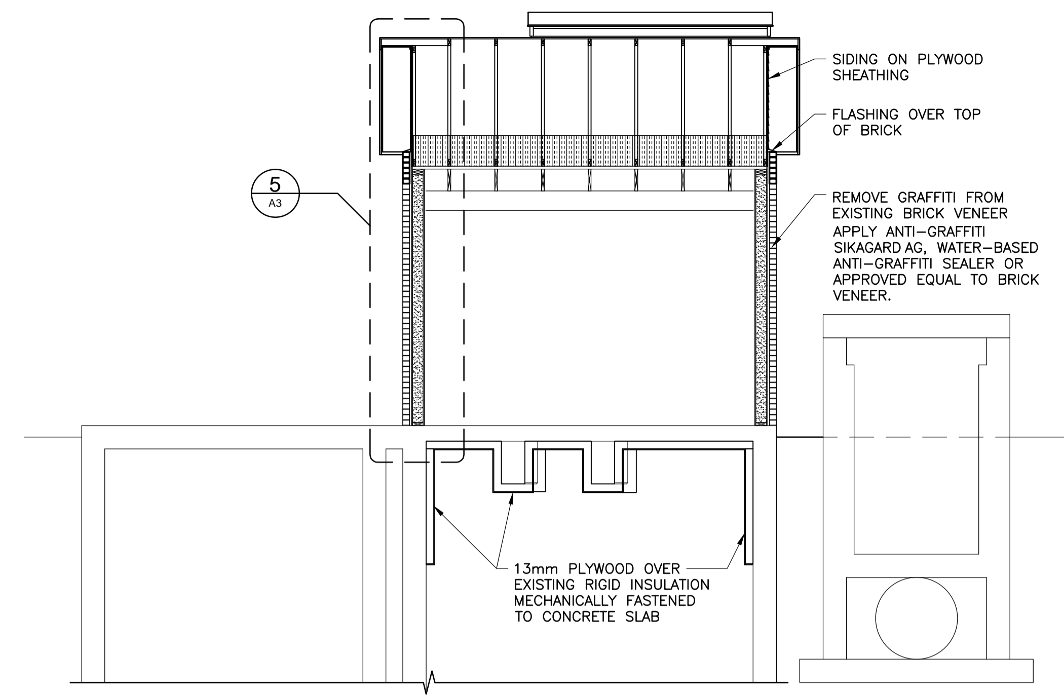
2 CROSS SECTION 1:50
