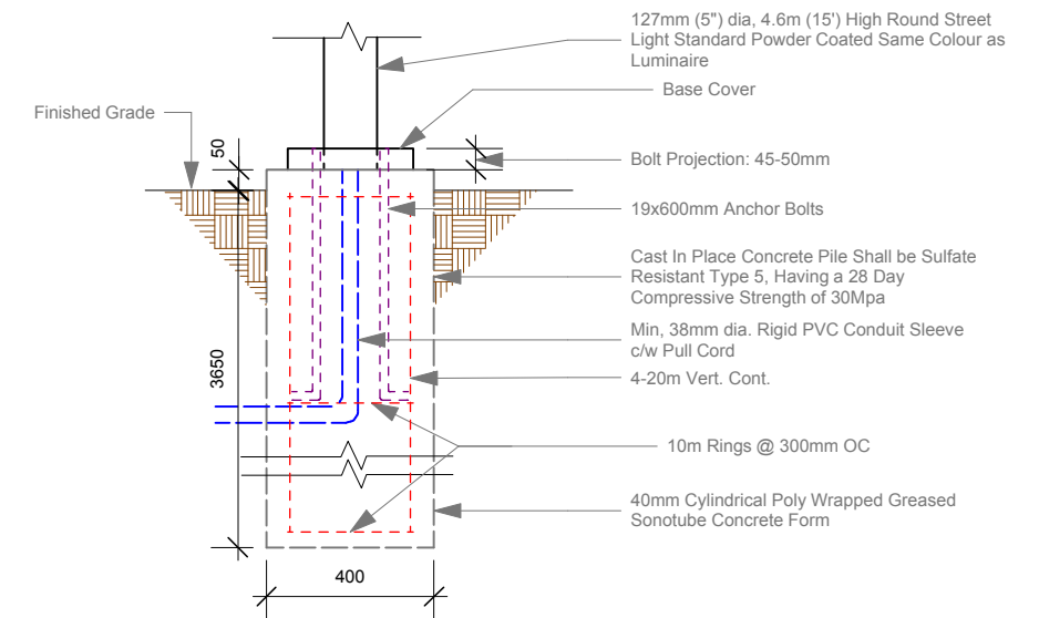
1 Lamp Standard Base Detail Scale: 1:20
