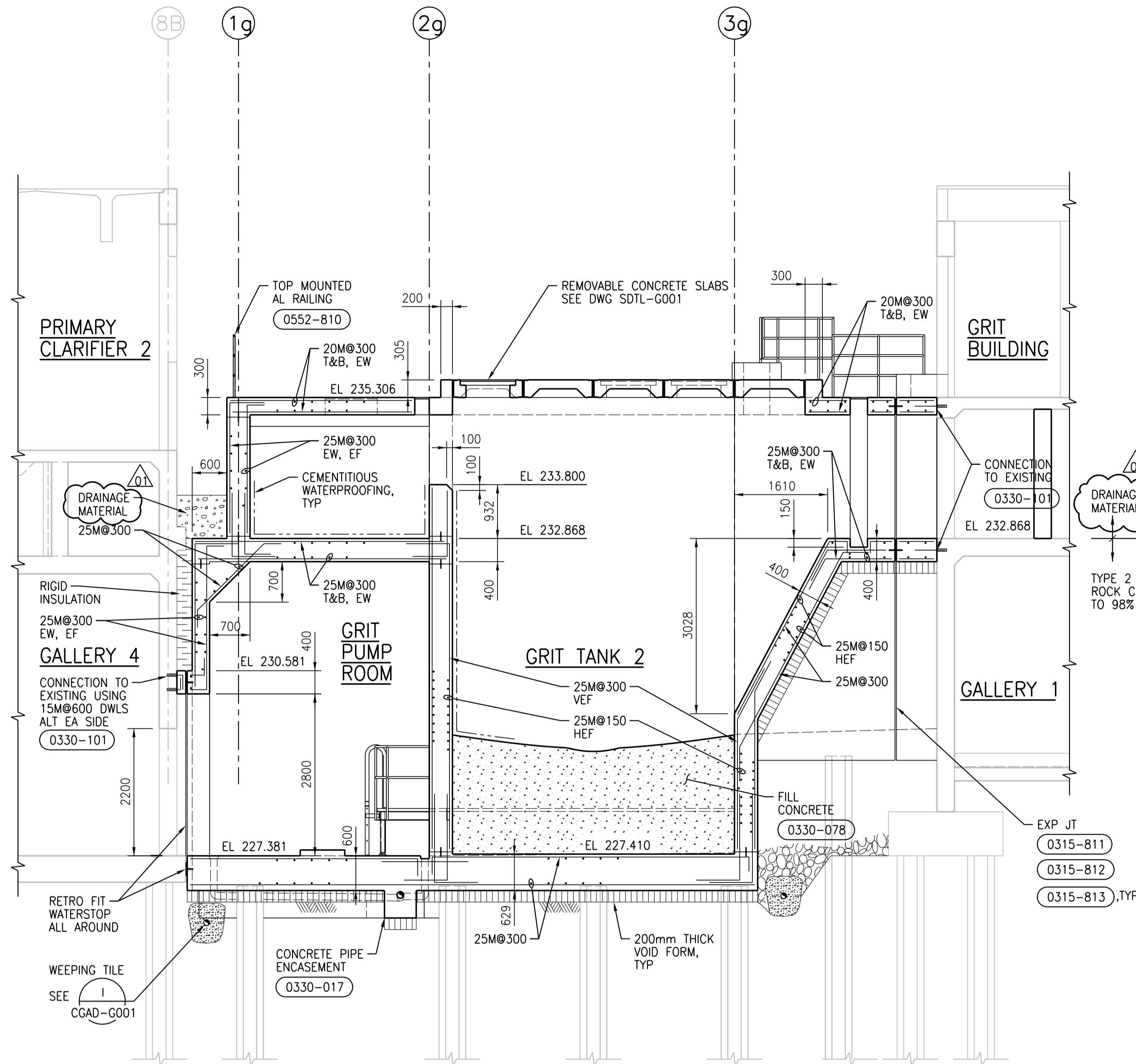
A SECTION 1:50 SGAD-G001, SGAD-G002, SGAD-G003
