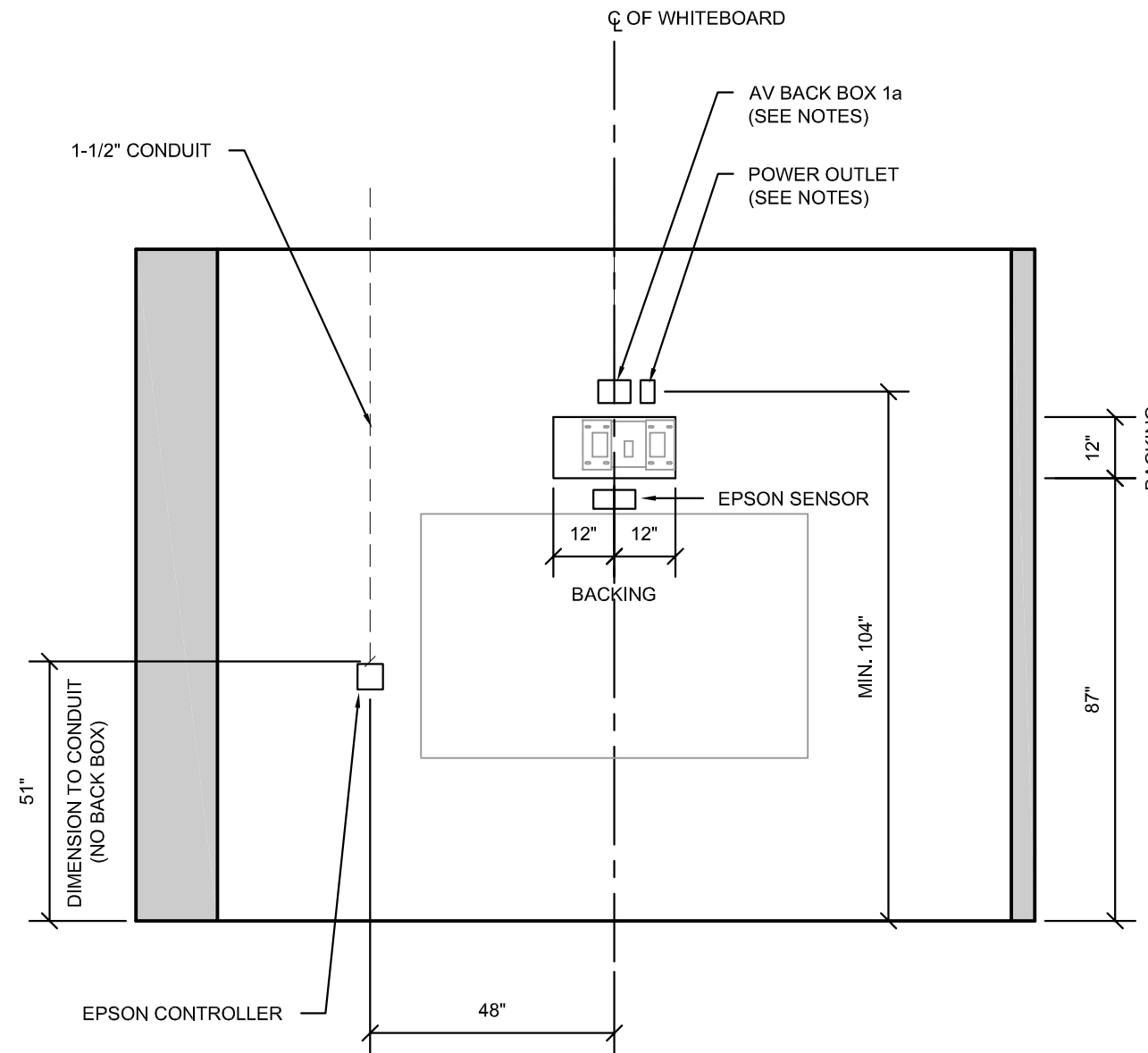
WEST WALL - BACKING, BACK BOX & CONDUIT DETAILS
