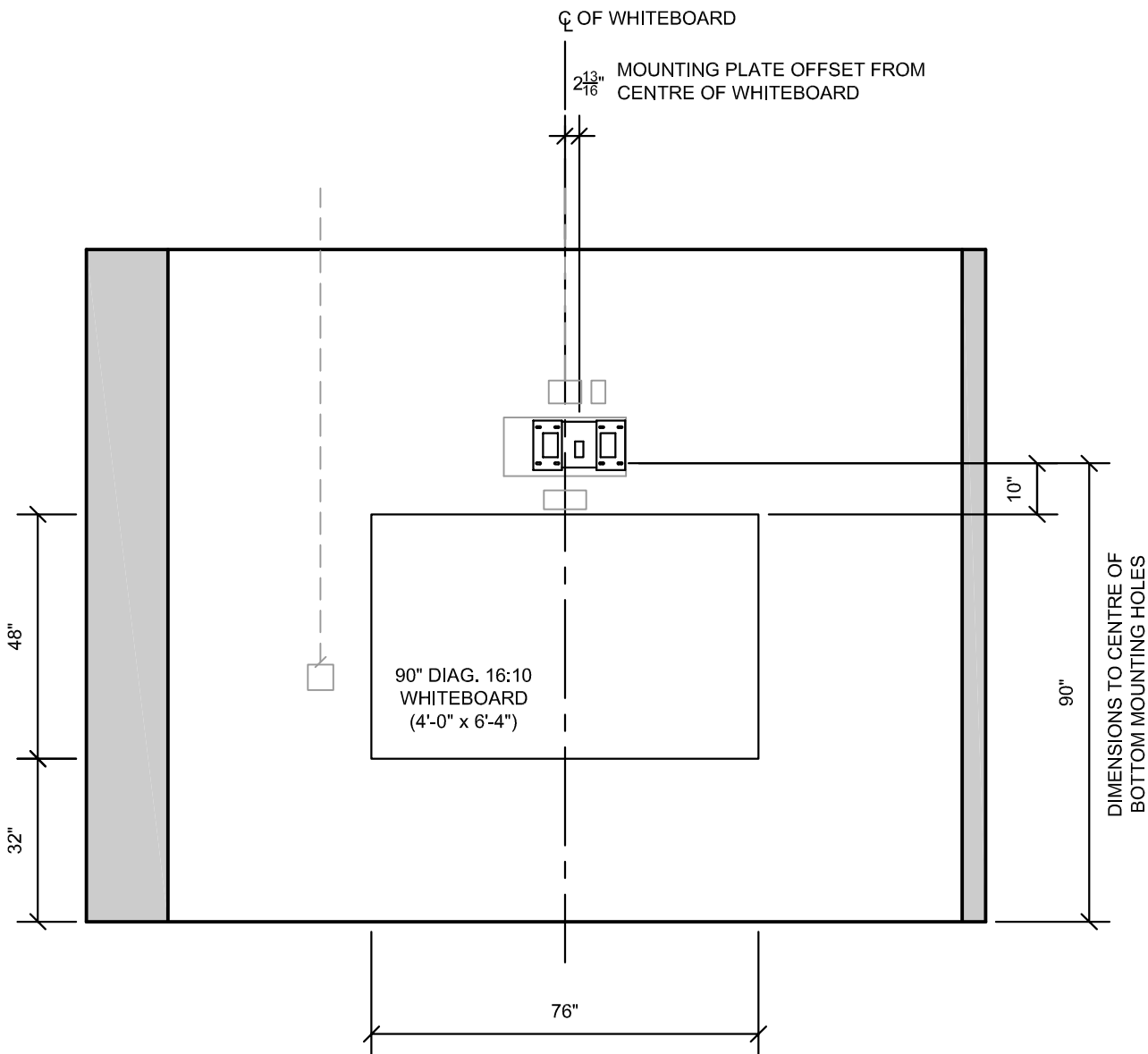
WEST WALL - SHOWING WHITEBOARD & WALL MOUNT DIMENSIONS
