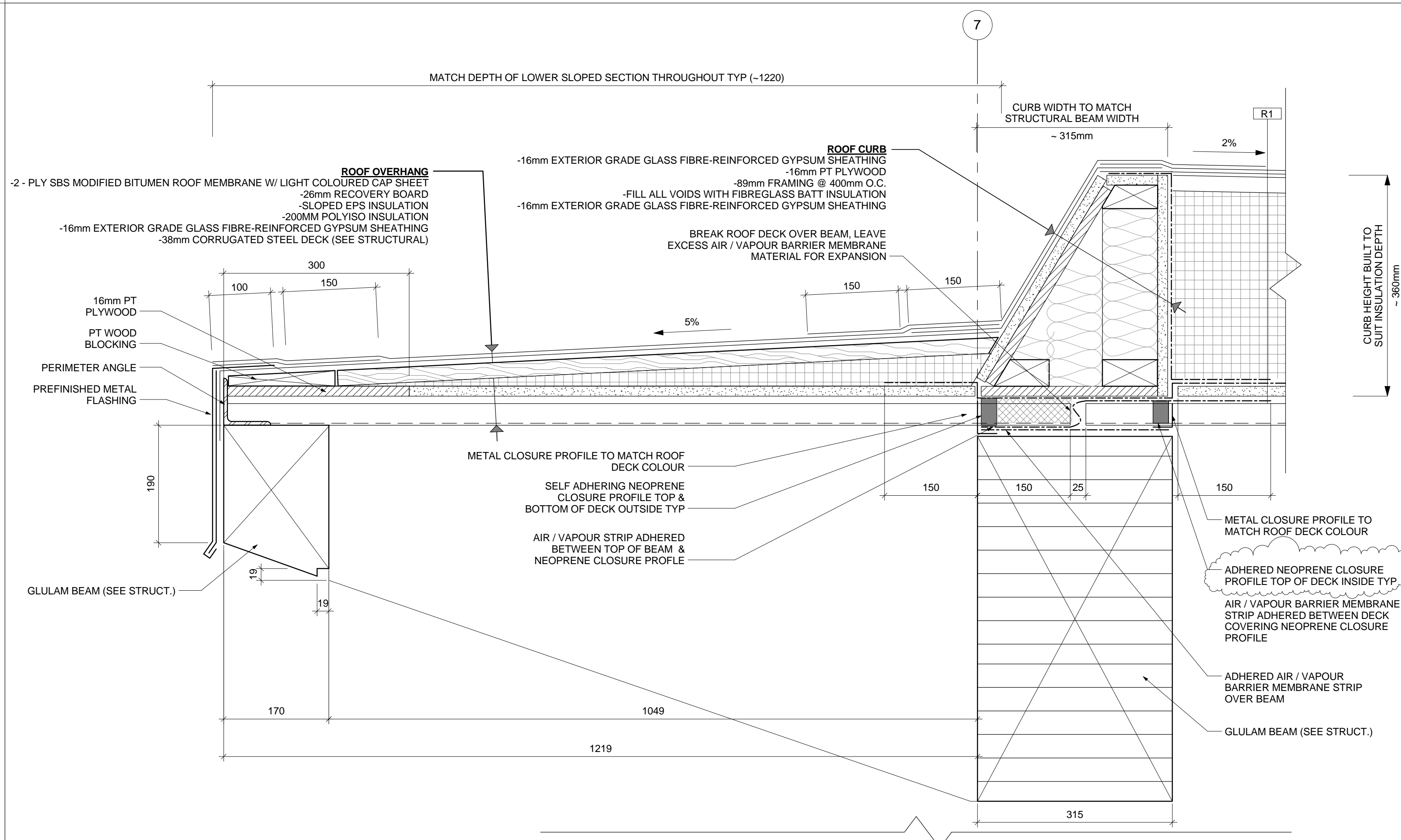
1 TYPICAL SECTION DETAIL - ROOF EDGE 1:5
