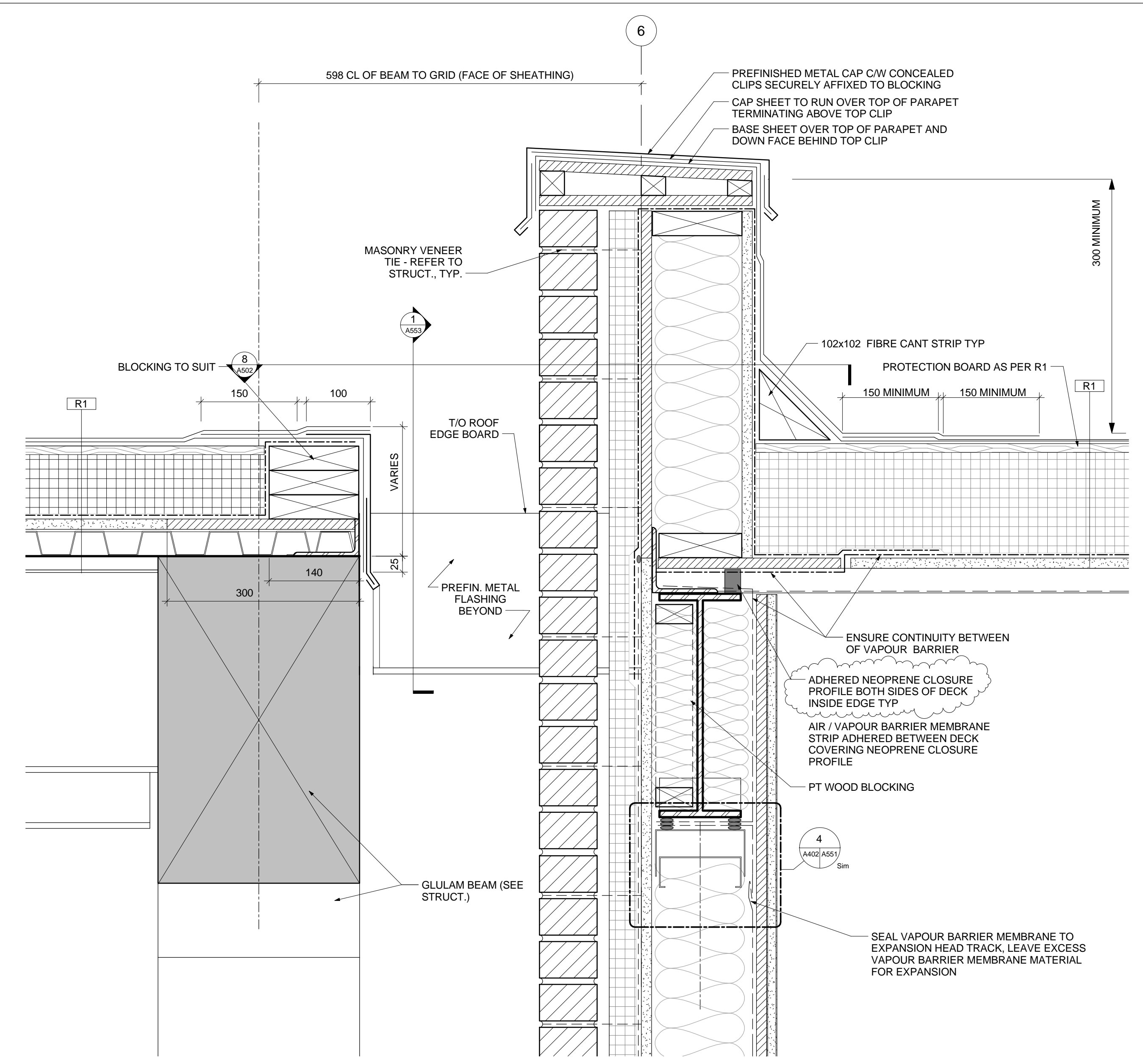
2 SECTION DETAIL - SLOPED ROOF @ FLAT ROOF 1:5
