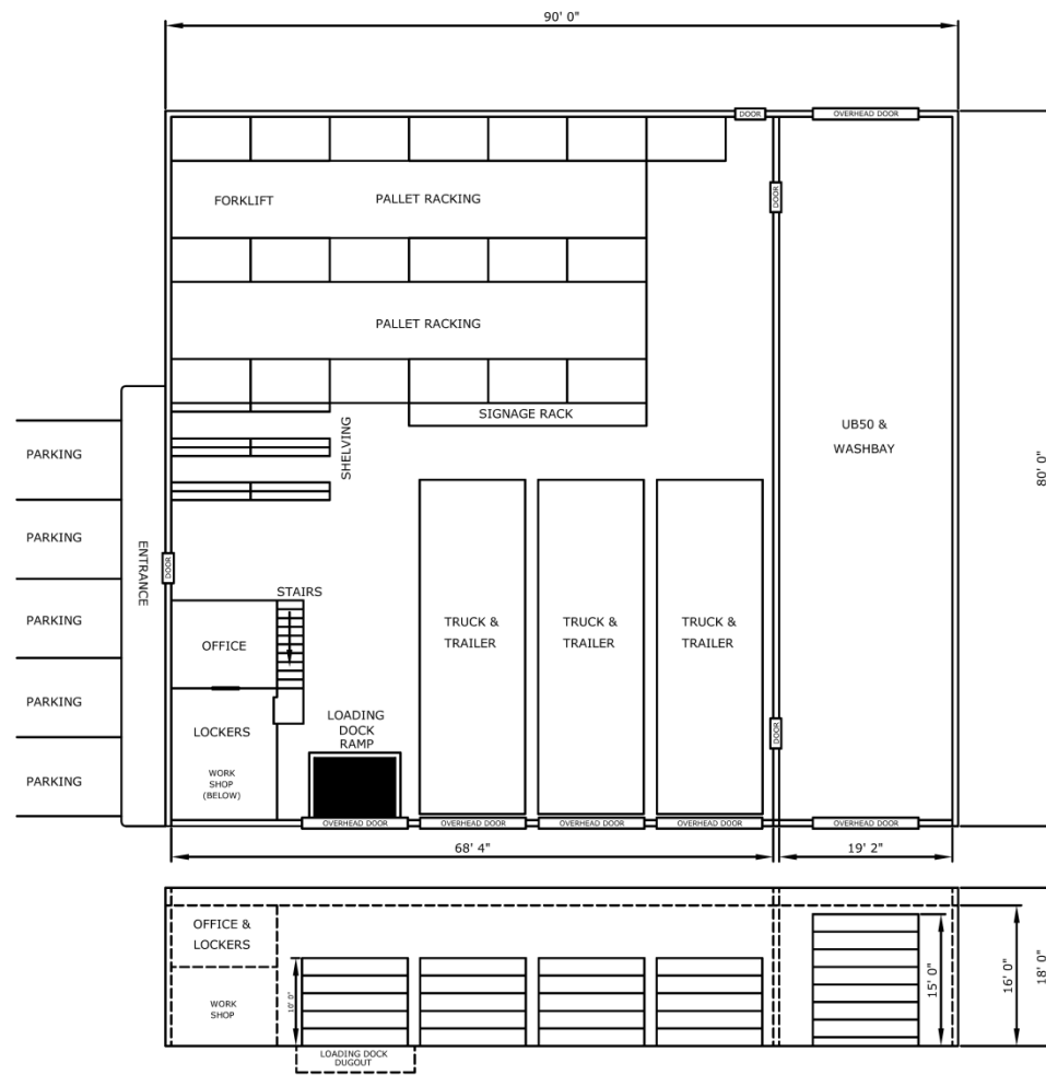
BRIDGE YARD BUILDING CONCEPT - OPTION #2
