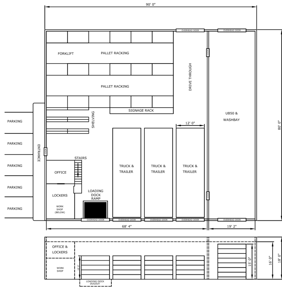
BRIDGE YARD BUILDING CONCEPT - OPTION #1
