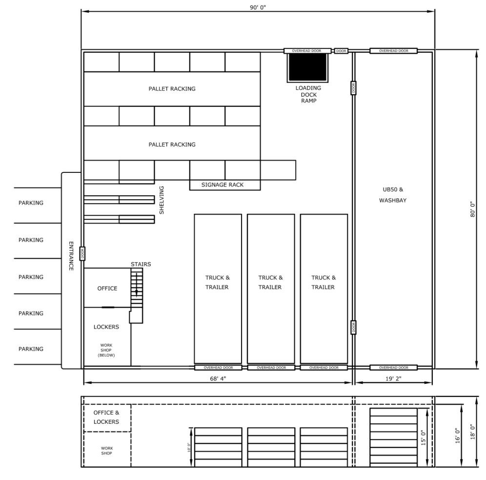
BRIDGE YARD BUILDING CONCEPT - OPTION #3
