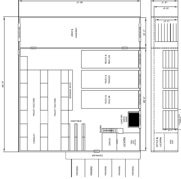
BRIDGE YARD BUILDING CONCEPT - OPTION #2
