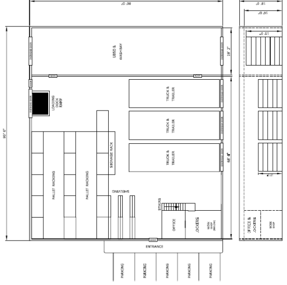
BRIDGE YARD BUILDING CONCEPT - OPTION #3
