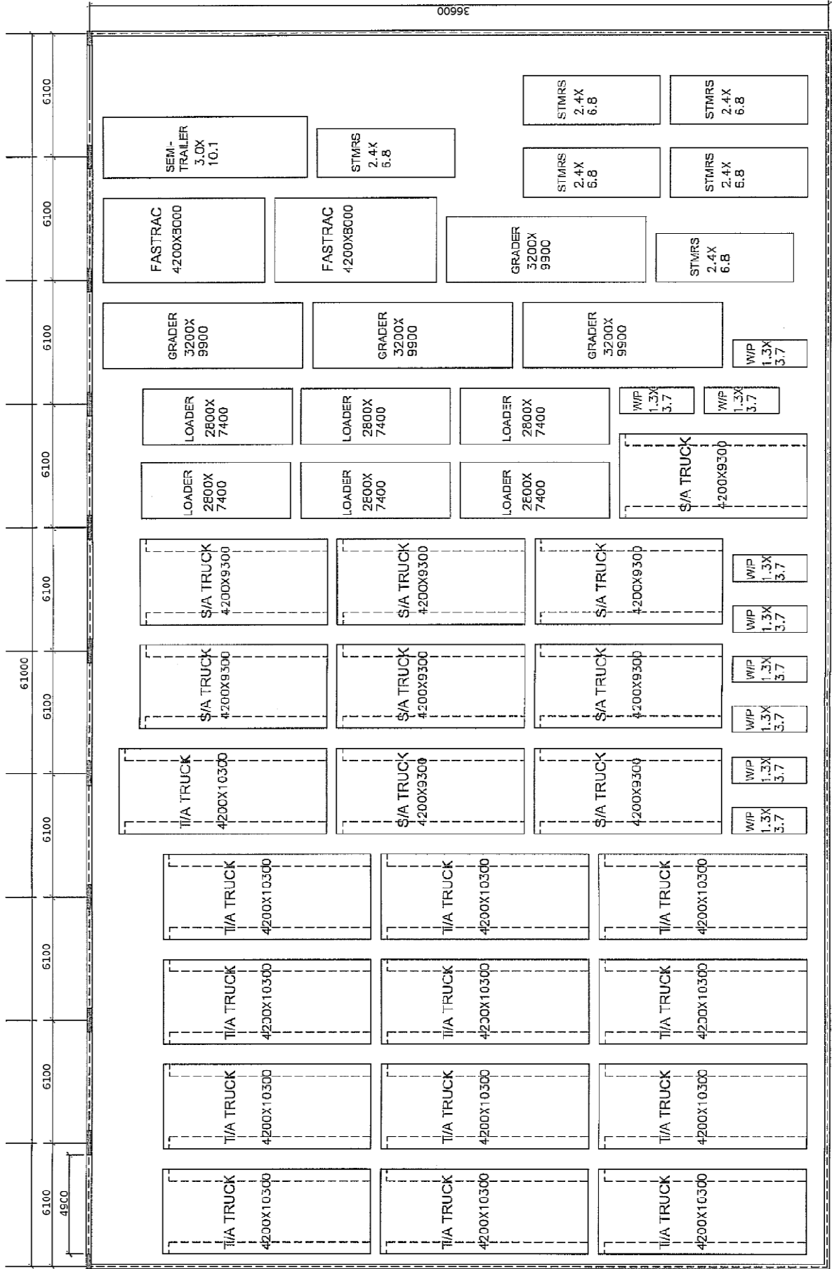
Figure C7R1 – Schematic Plan for Streets Maintenance Heated Vehicle and Equipment Storage (SM-09)
