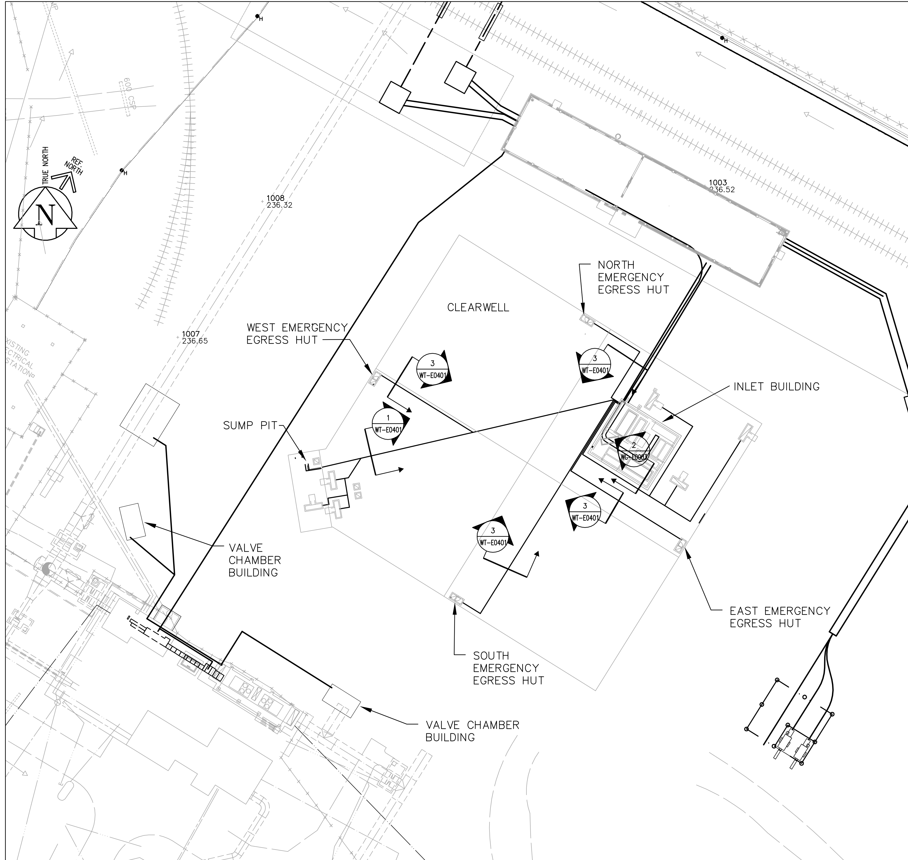
PARTIAL ELECTRICAL SITE PLAN 1:400
