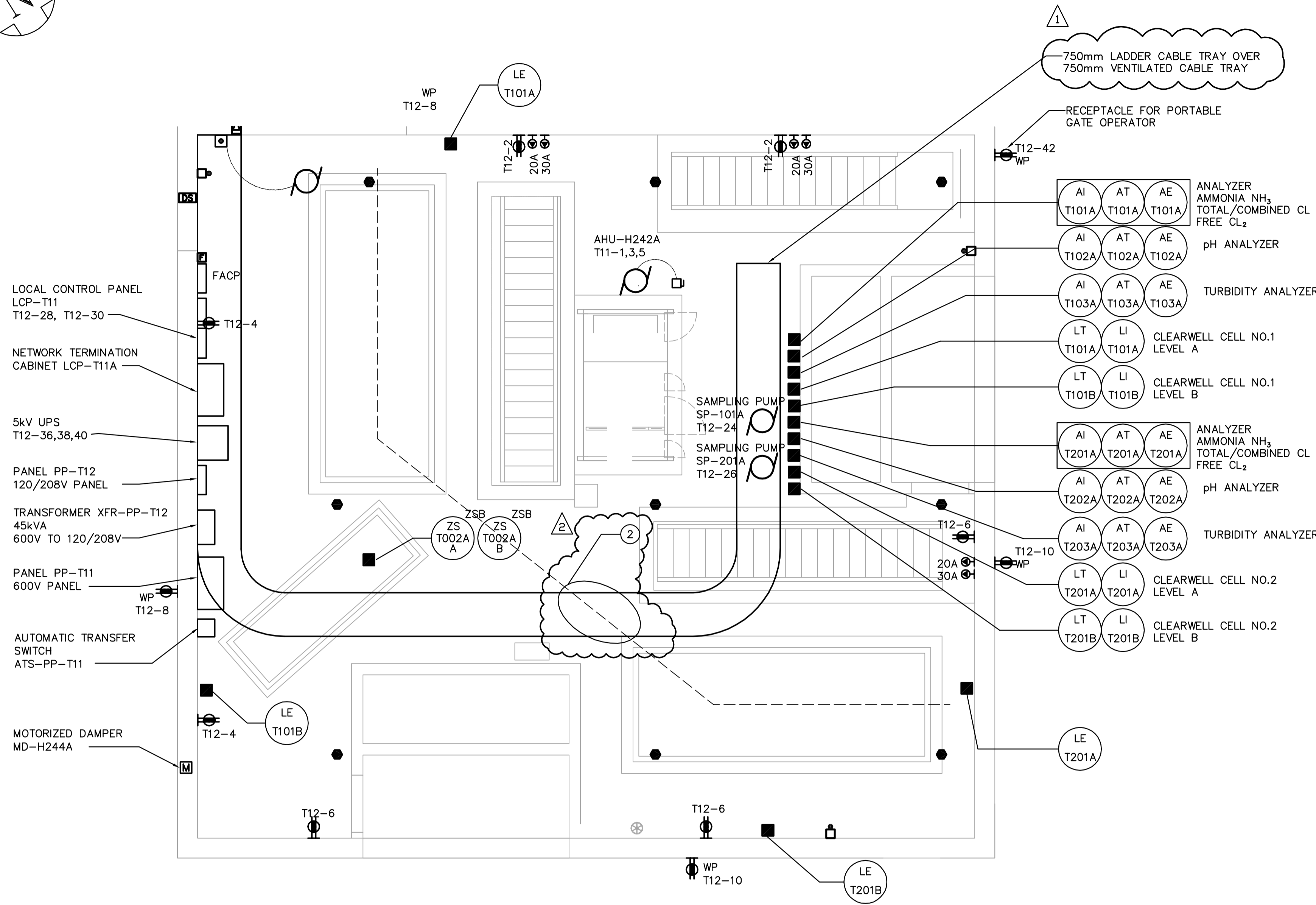
INLET BUILDING MAIN FLOOR POWER PLAN 1:50
