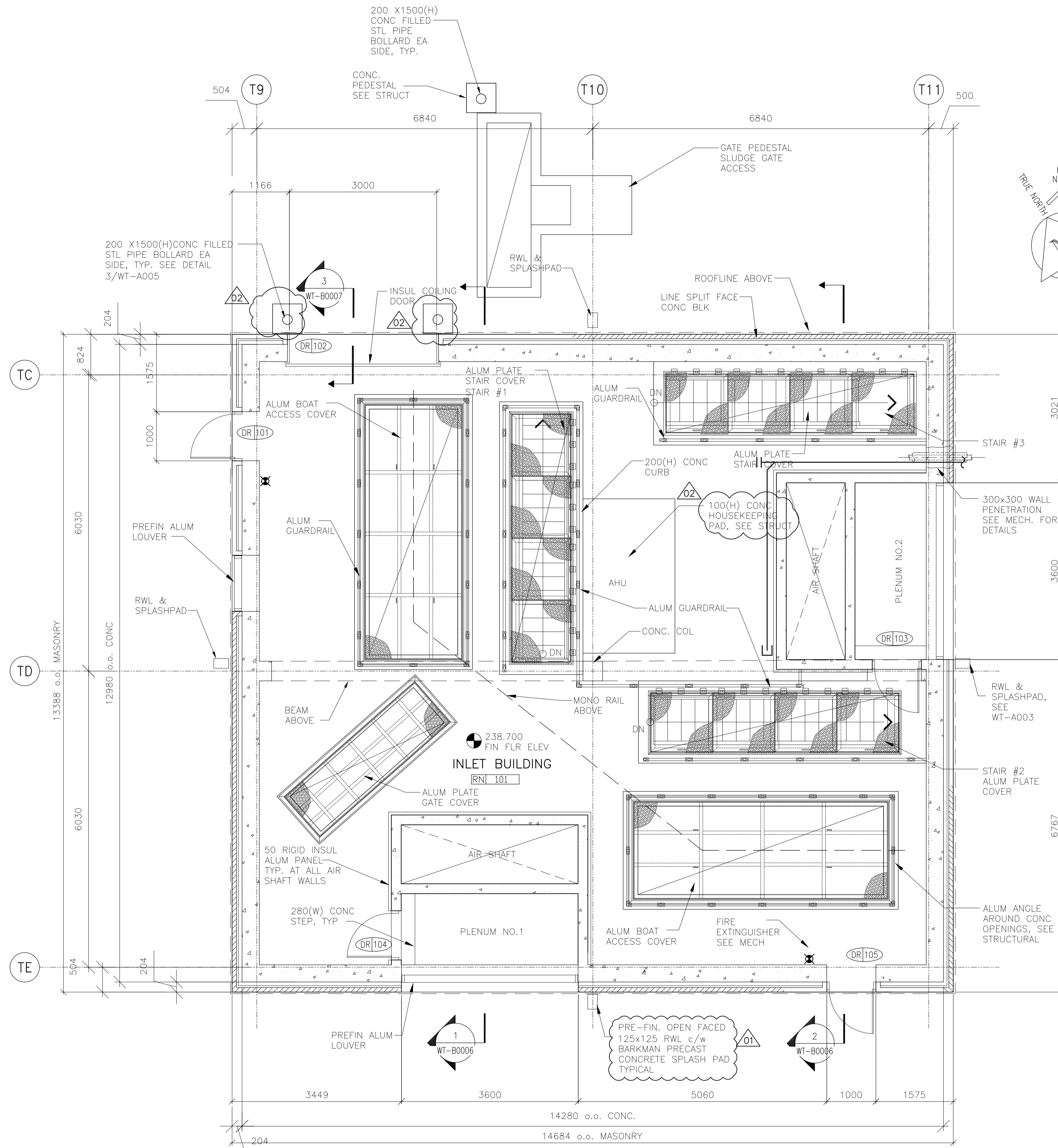
1 INLET BUILDING FLOOR PLAN AT ELEV: 238.700 1:50
