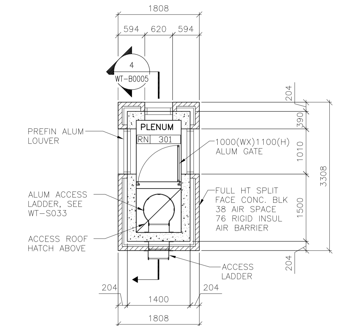
2 EMERGENCY EGRESS HUT FLOOR PLAN- TYPICAL OF 4 1:50
