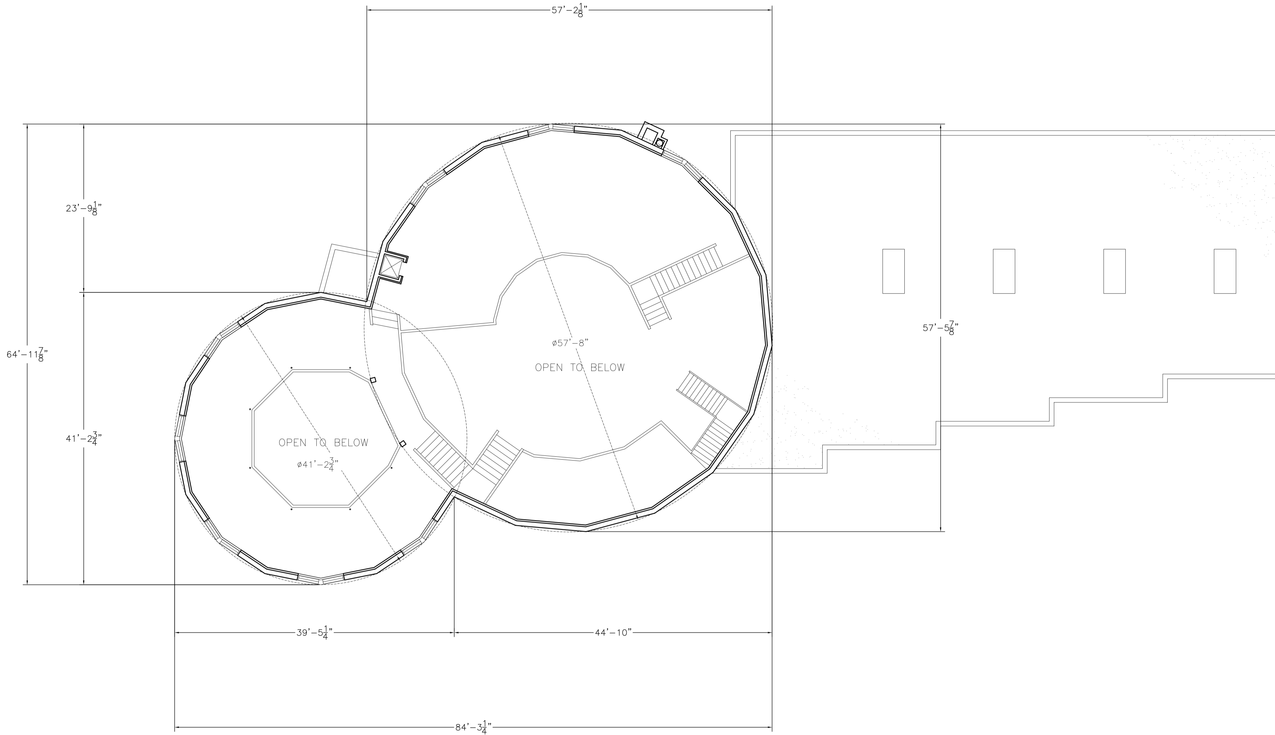
MEZZANINE FLOOR PLAN
