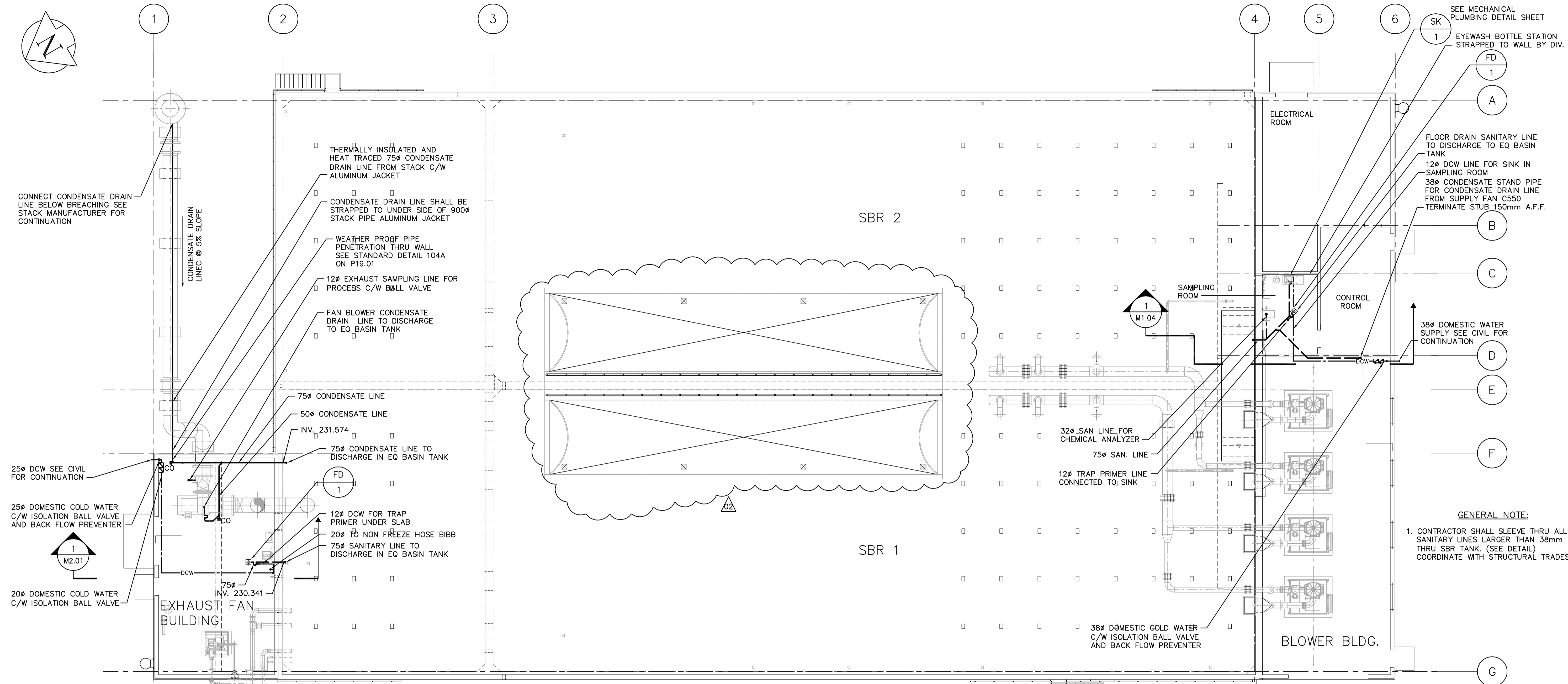
1 SBR, BLOWER BLDG & EXHAUST BLDG - PLUMBING PLAN M1.01 SCALE 1:100
