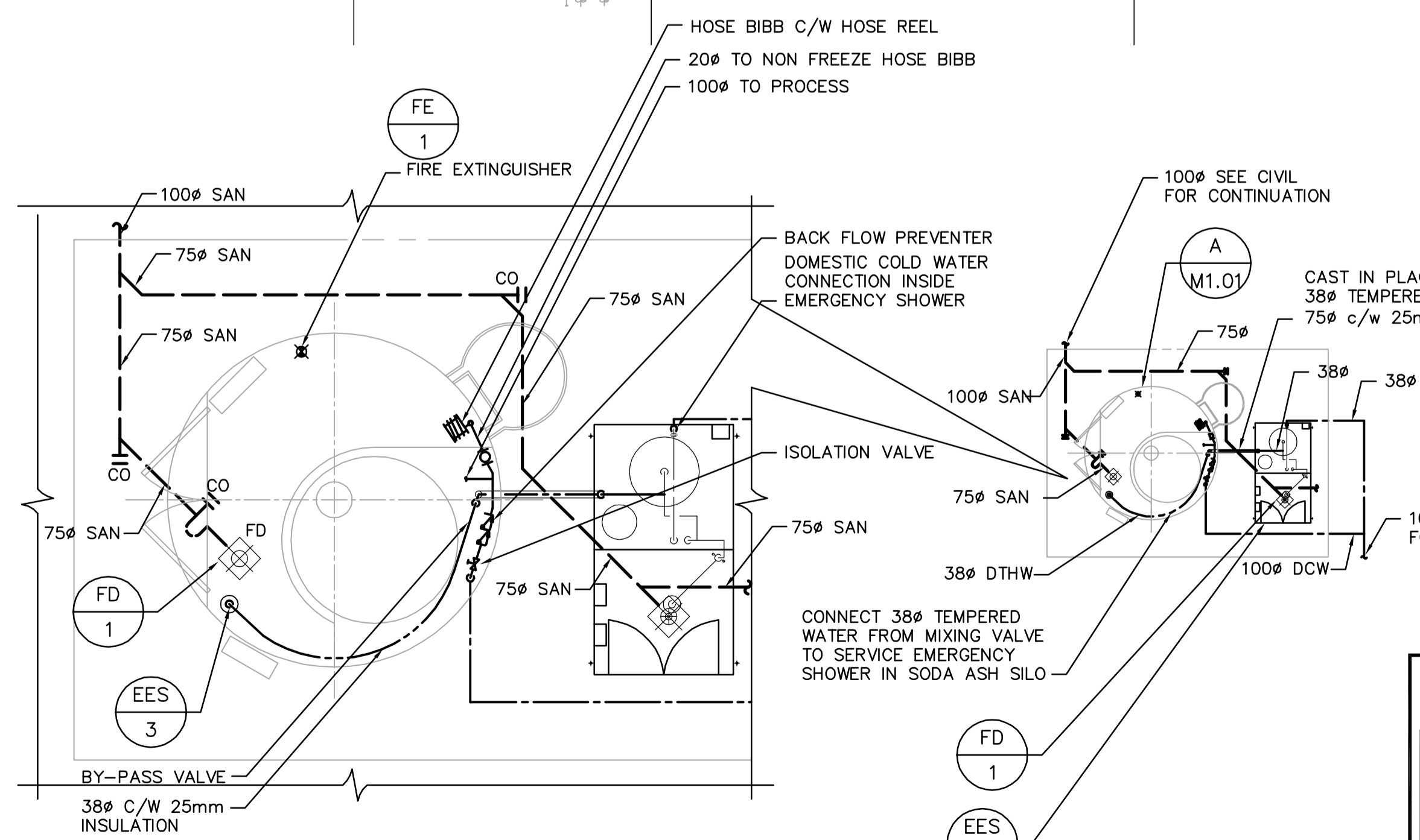
A SODA ASH DETAIL M1.01 SCALE 1:50
