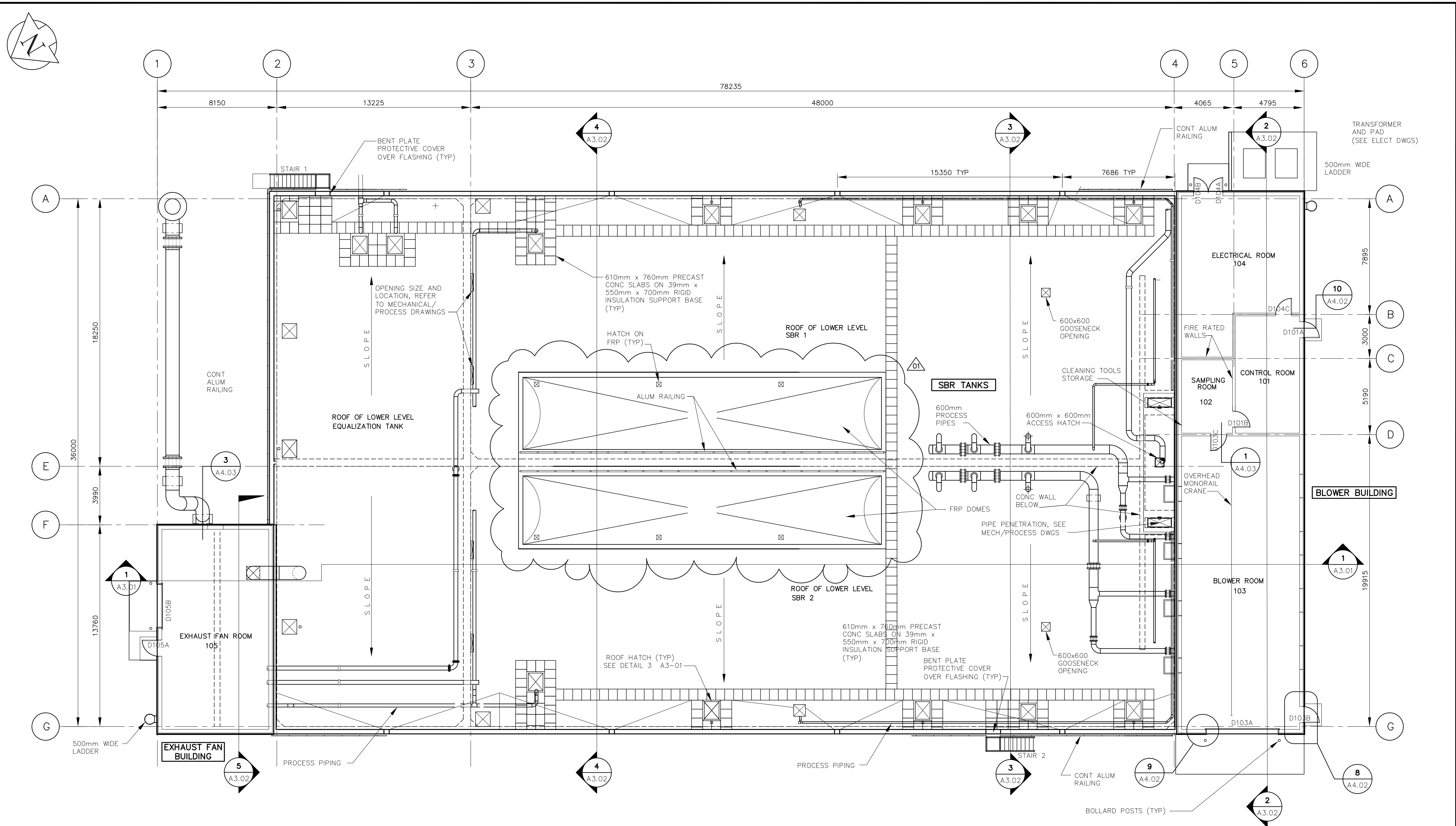
1 UPPER LEVEL PLAN A1.02 1:125
