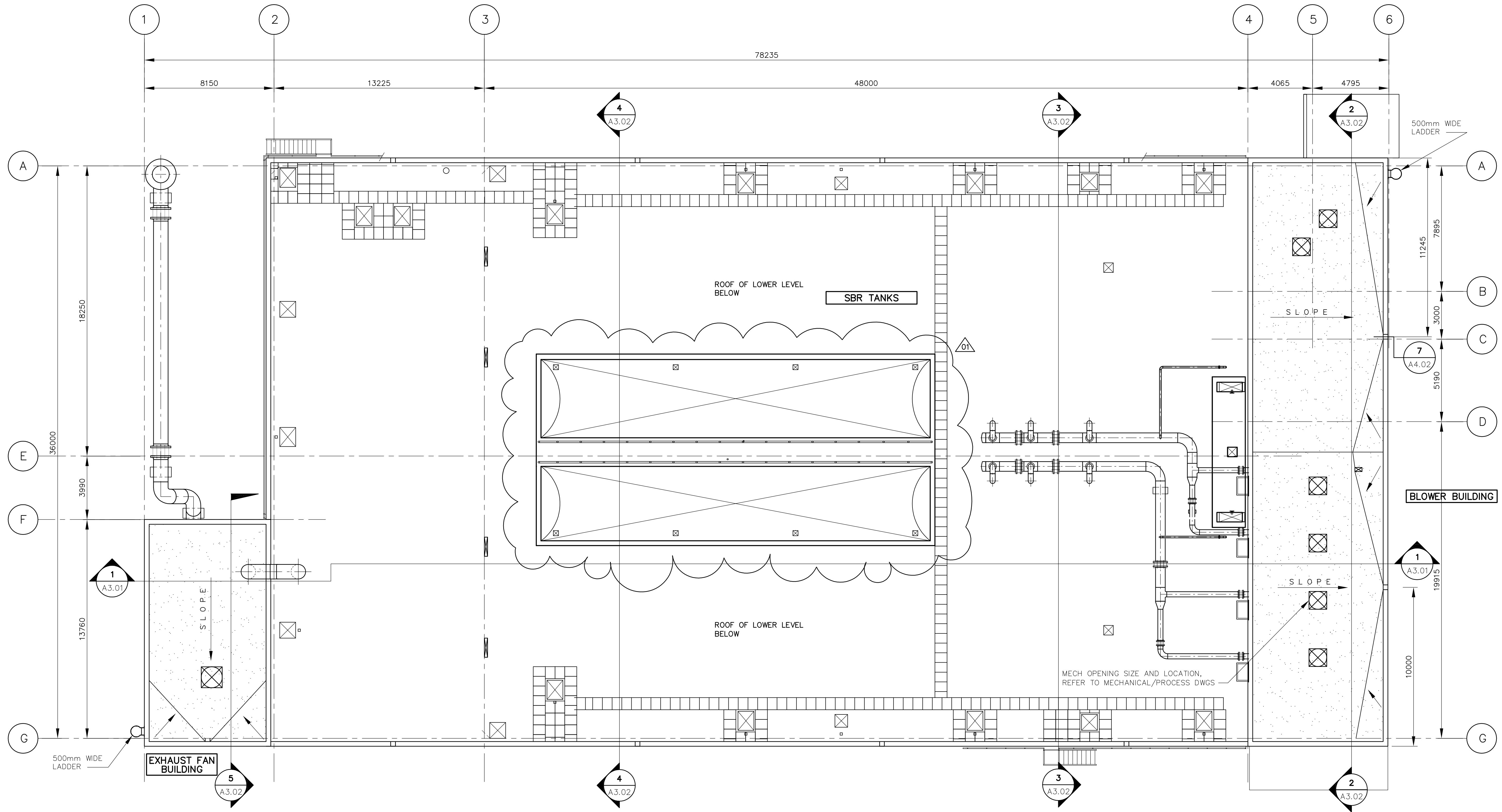
1 UPPER ROOF PLAN A1.01 1:125
