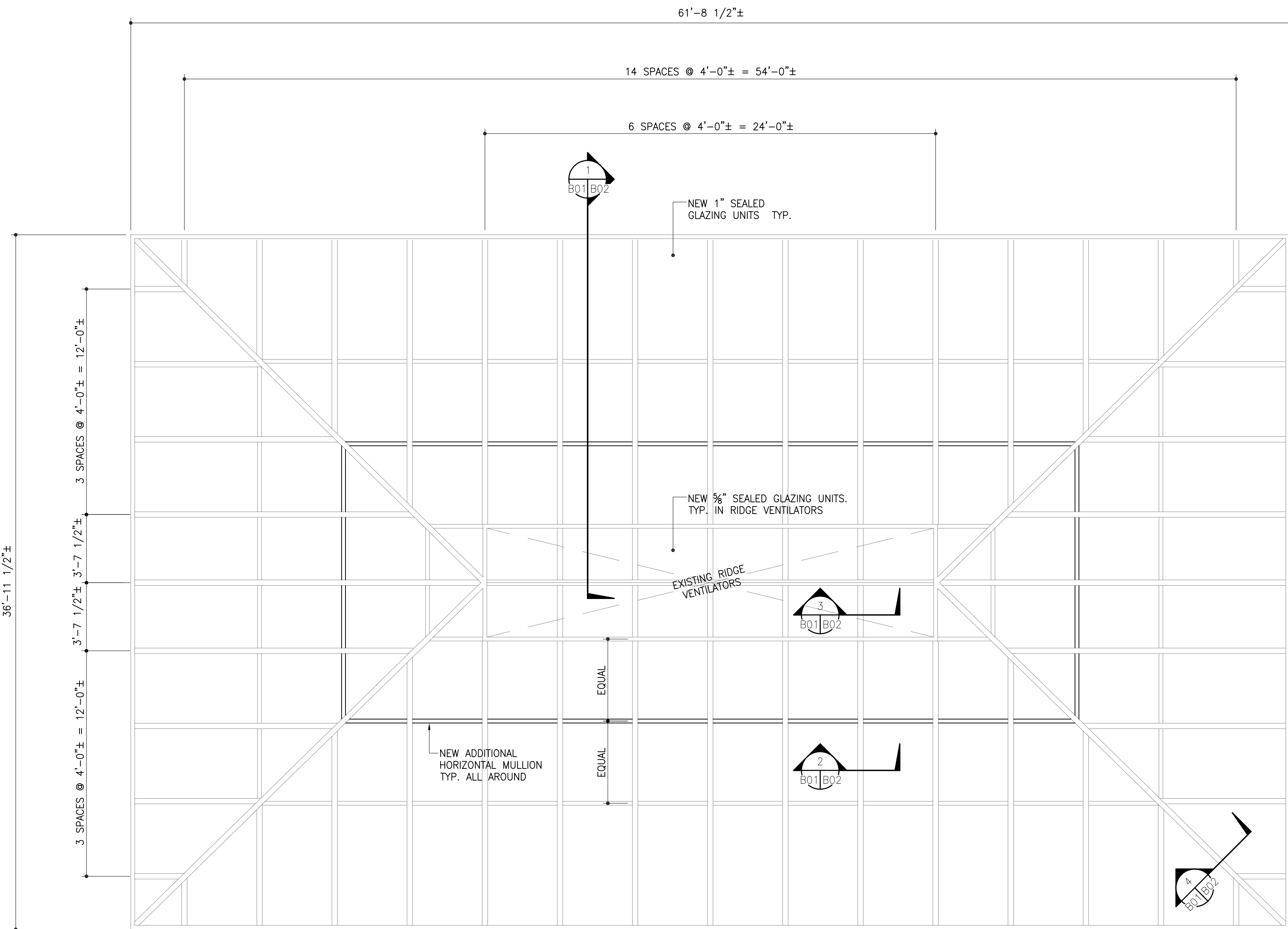
A EXISTING DISPLAY HOUSE SKYLIGHT ROOF PLAN B01|B01 1/4"=1'-0"
