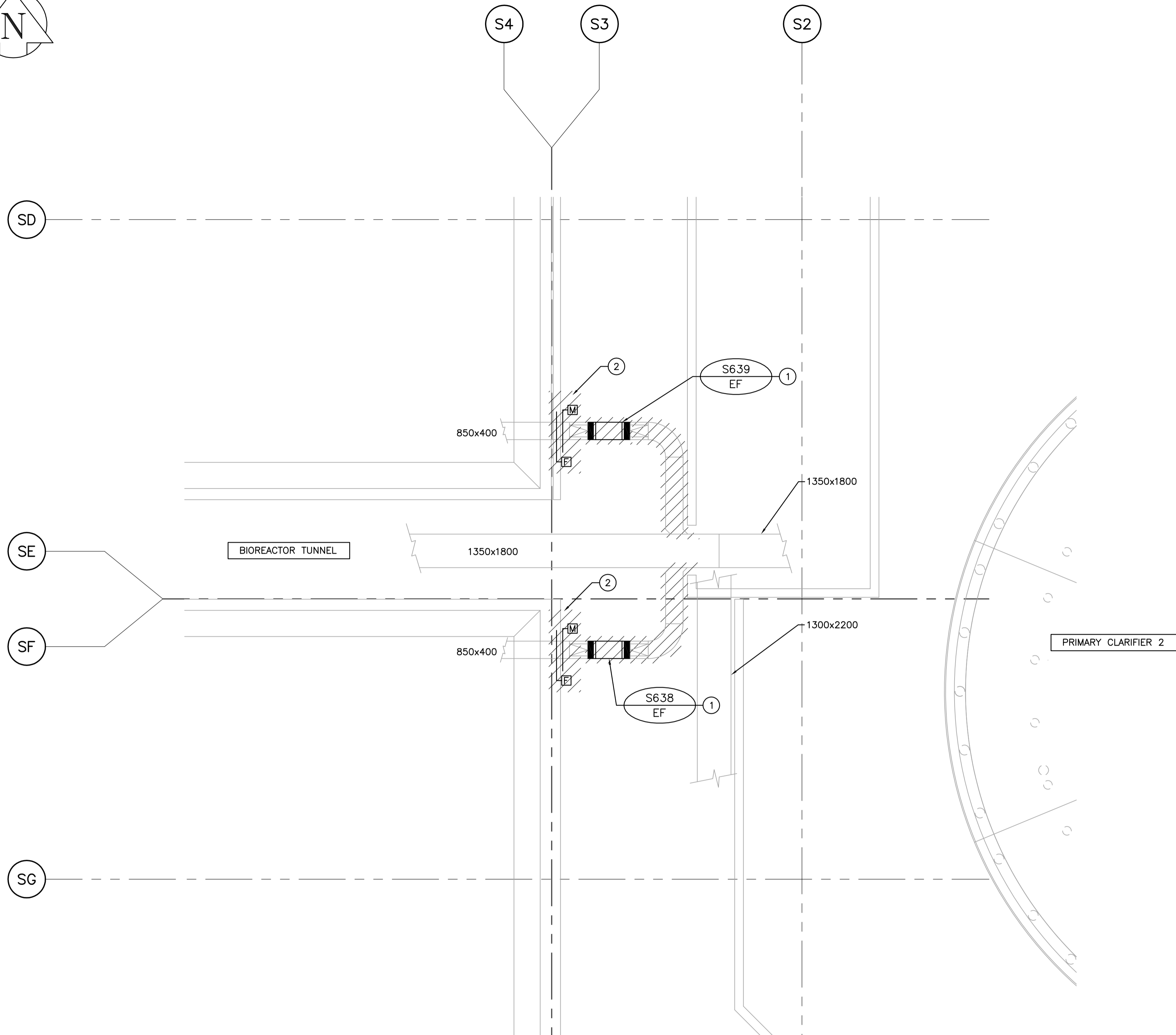
LOWER LEVEL – EXISTING VENTILATION DEMOLITION PLAN SCALE: 1:100
