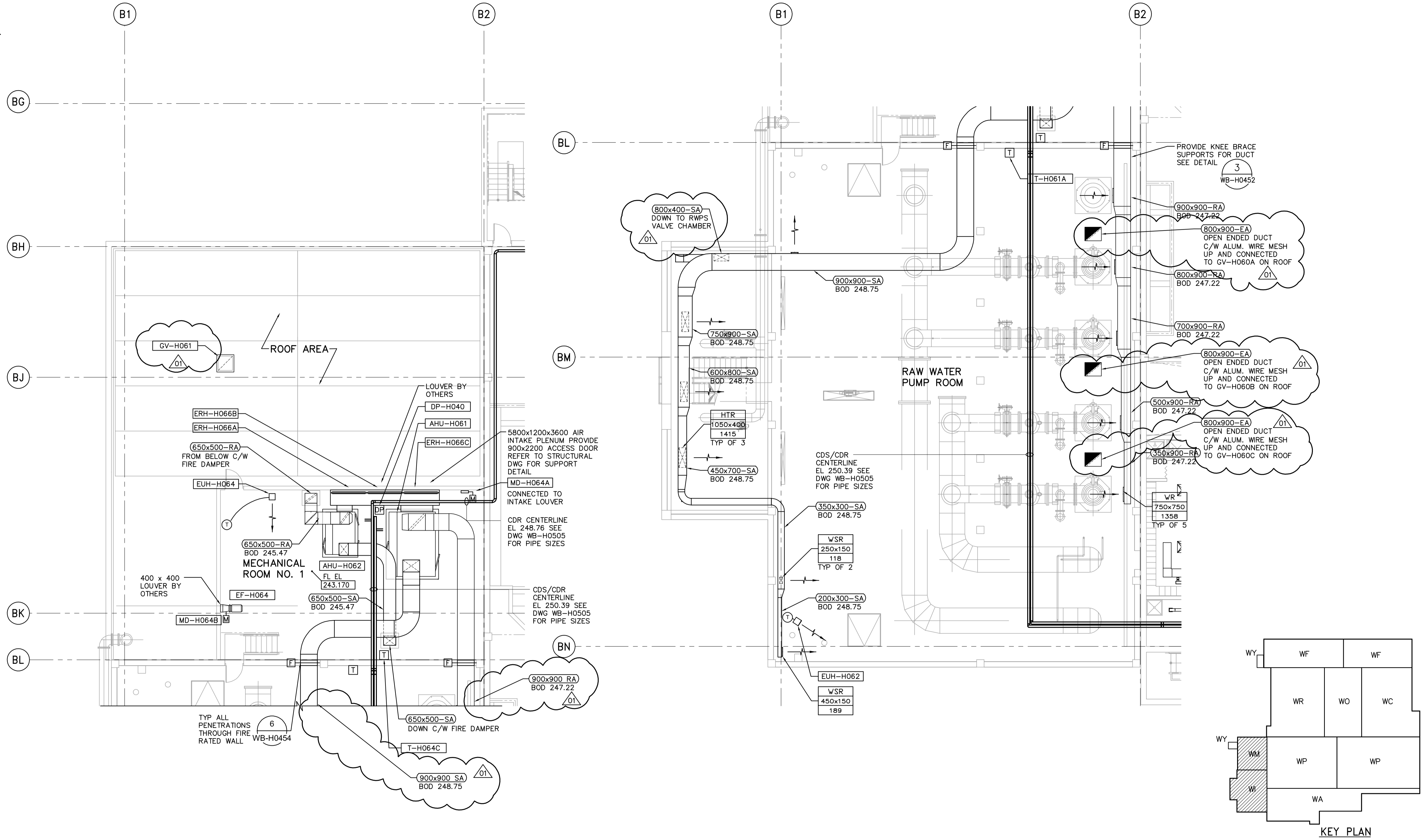
THIRD FLOOR PLAN 1:100
