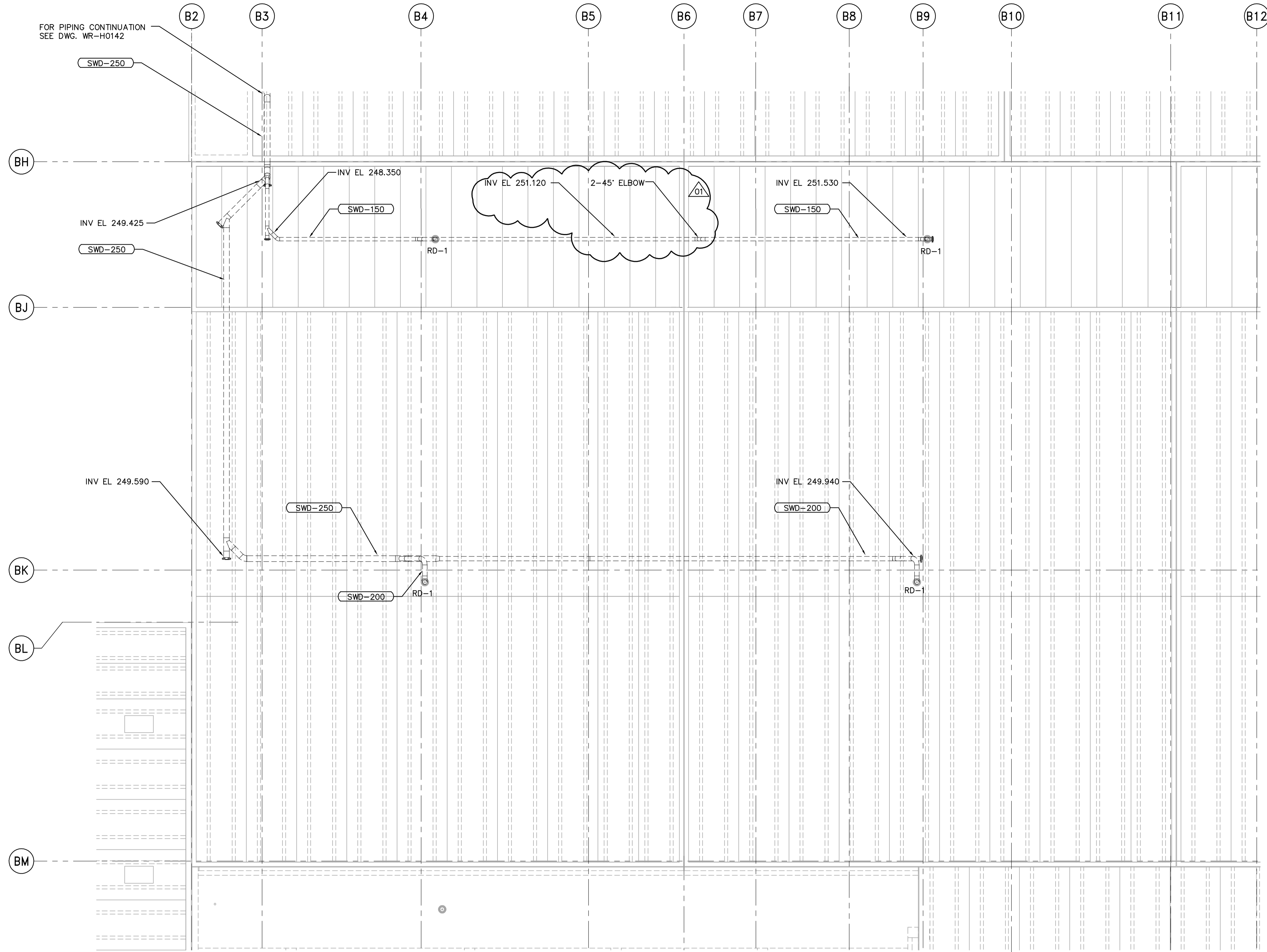
ROOF PLAN 1:100
