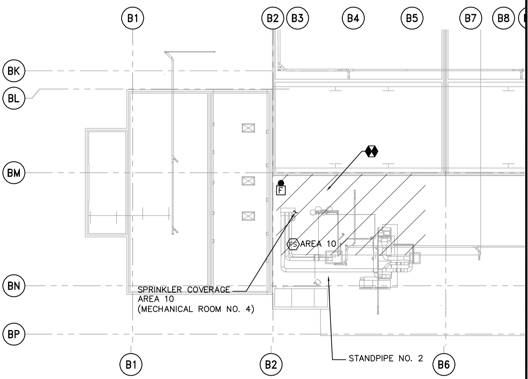
PARTIAL PLAN AT ELEVATION 251.450 1:300
