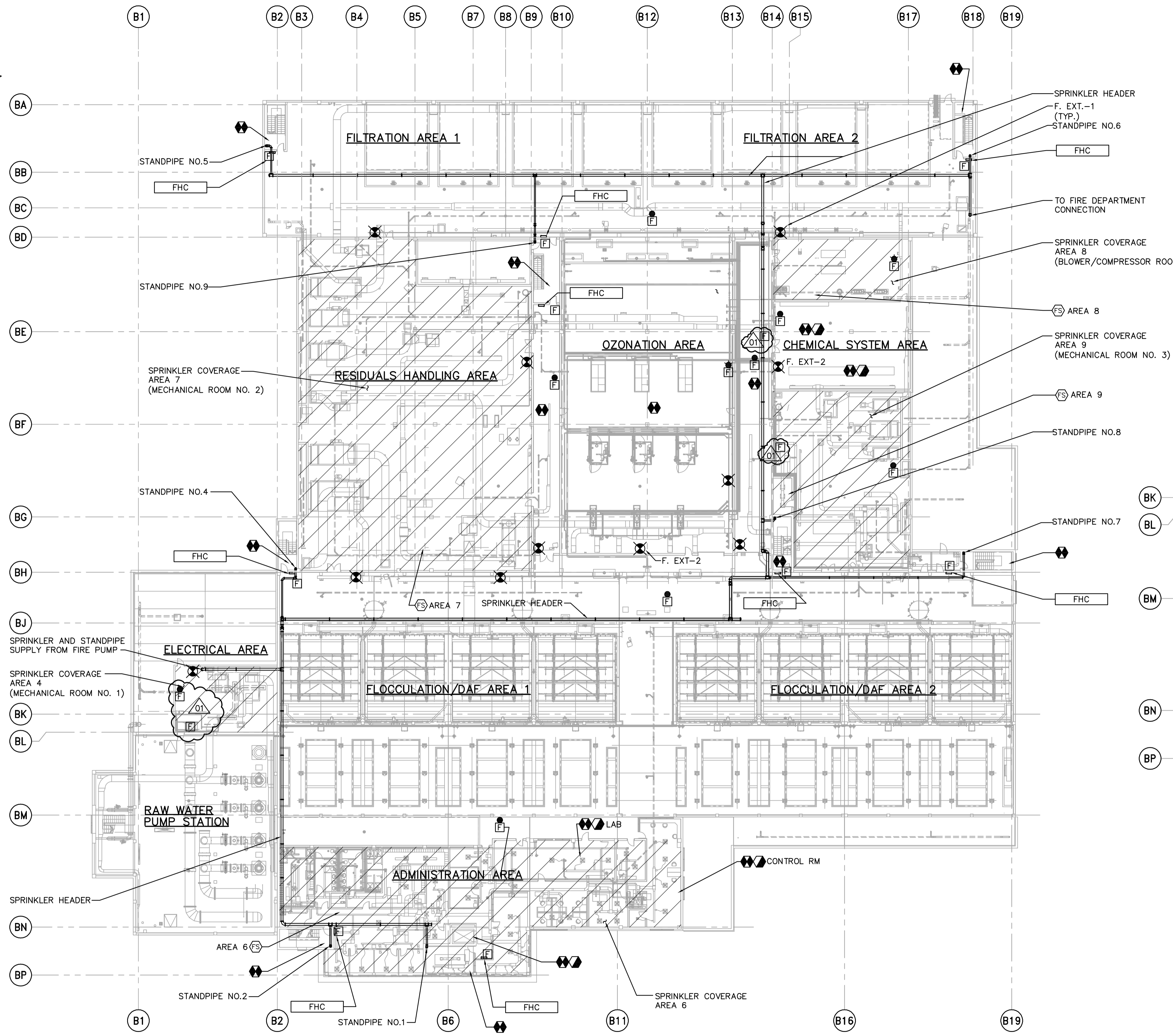
THIRD FLOOR PLAN 1:300
