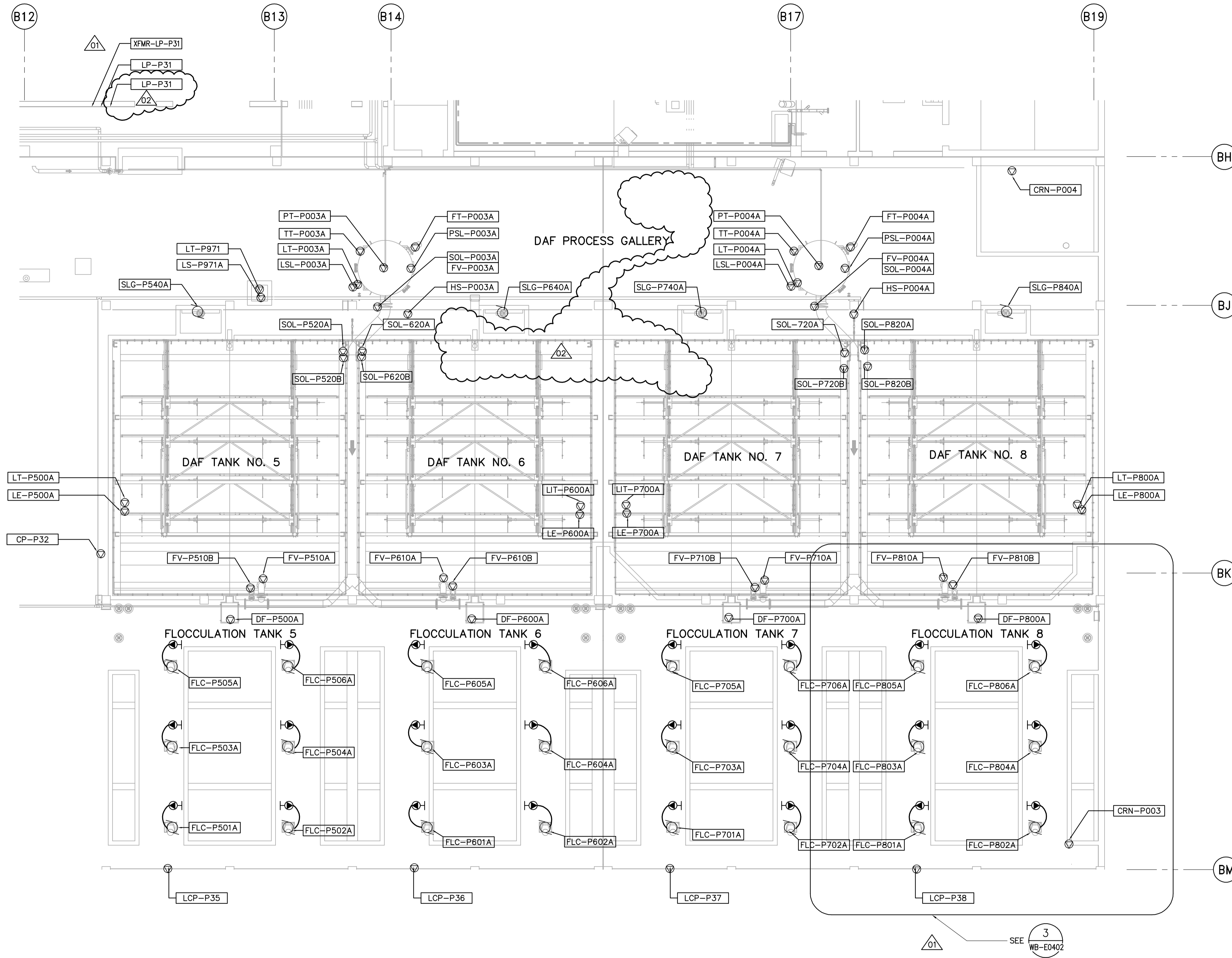
THIRD FLOOR PROCESS PLAN (AREA 2) 1:100
