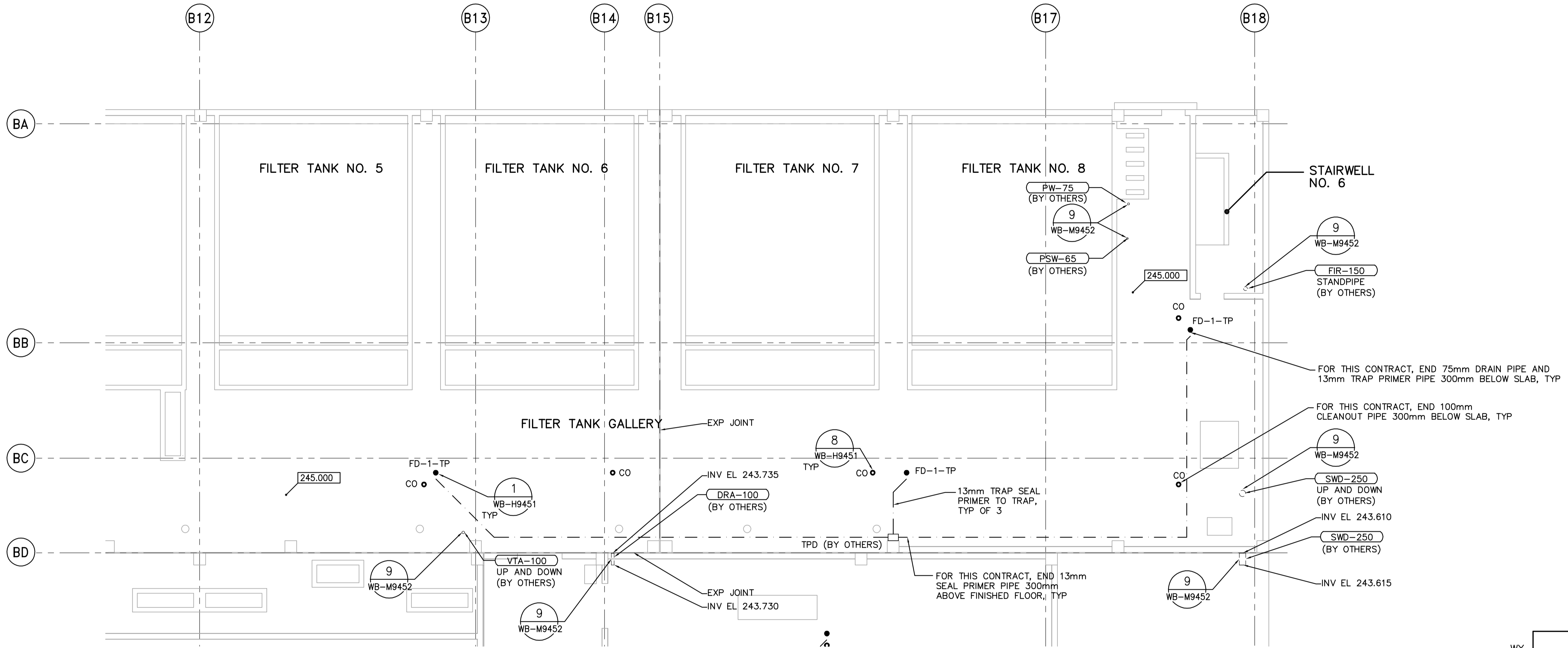
THIRD FLOOR PLAN 1:100
