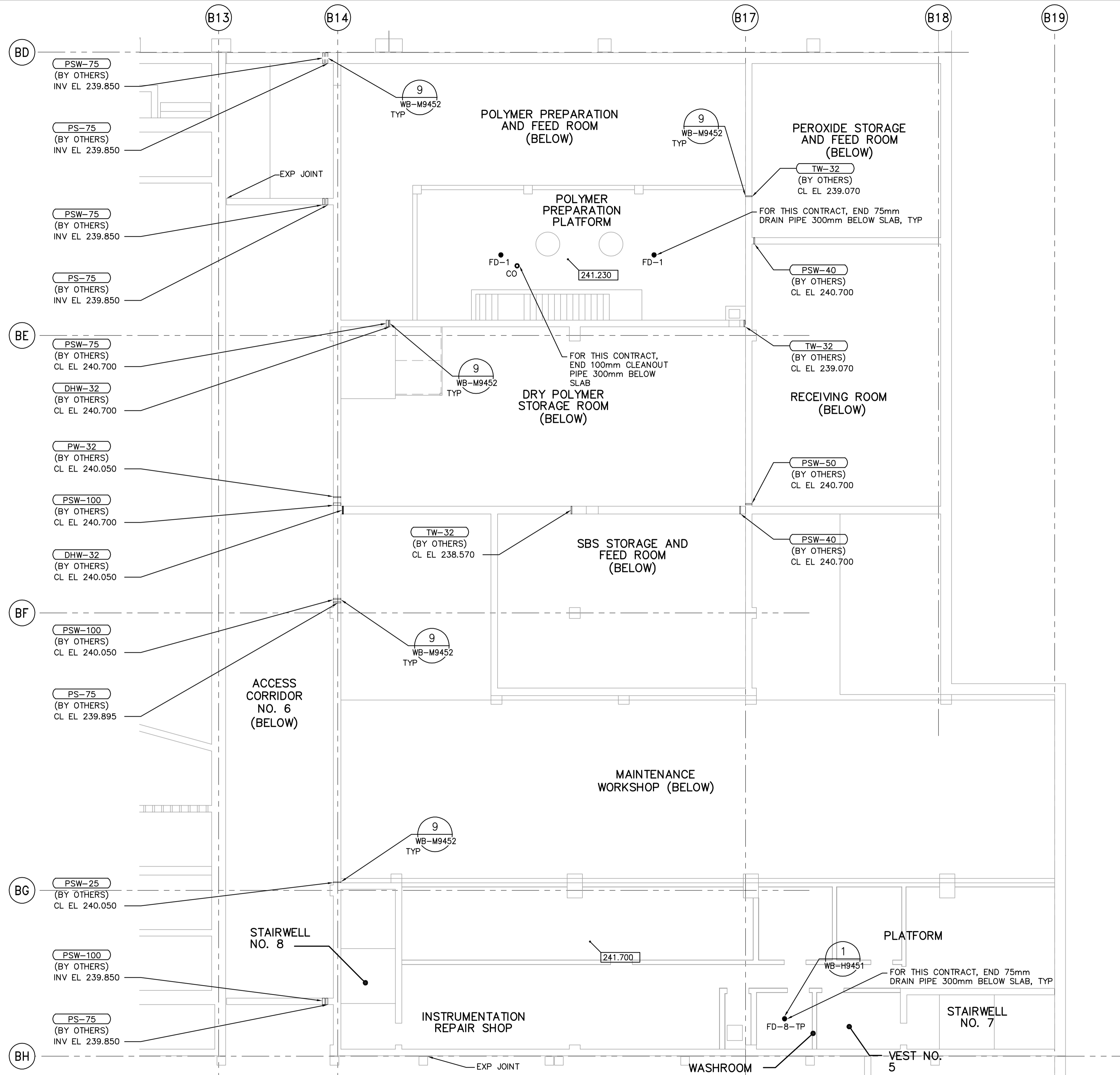
SECOND FLOOR PLAN 1:100
