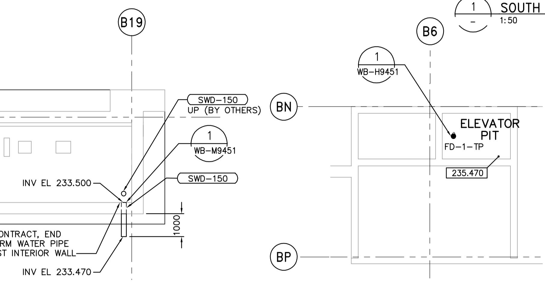
PARTIAL FIRST FLOOR PLAN 1:100
