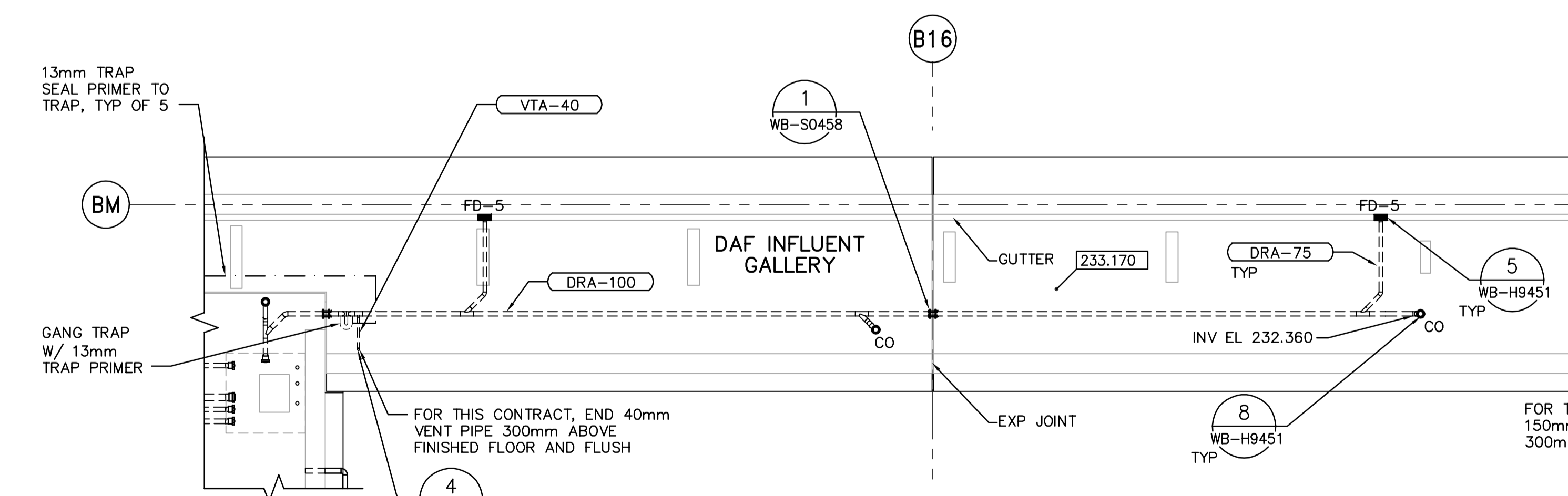
LOWER LEVEL PLAN (CONTINUATION) 1:100
