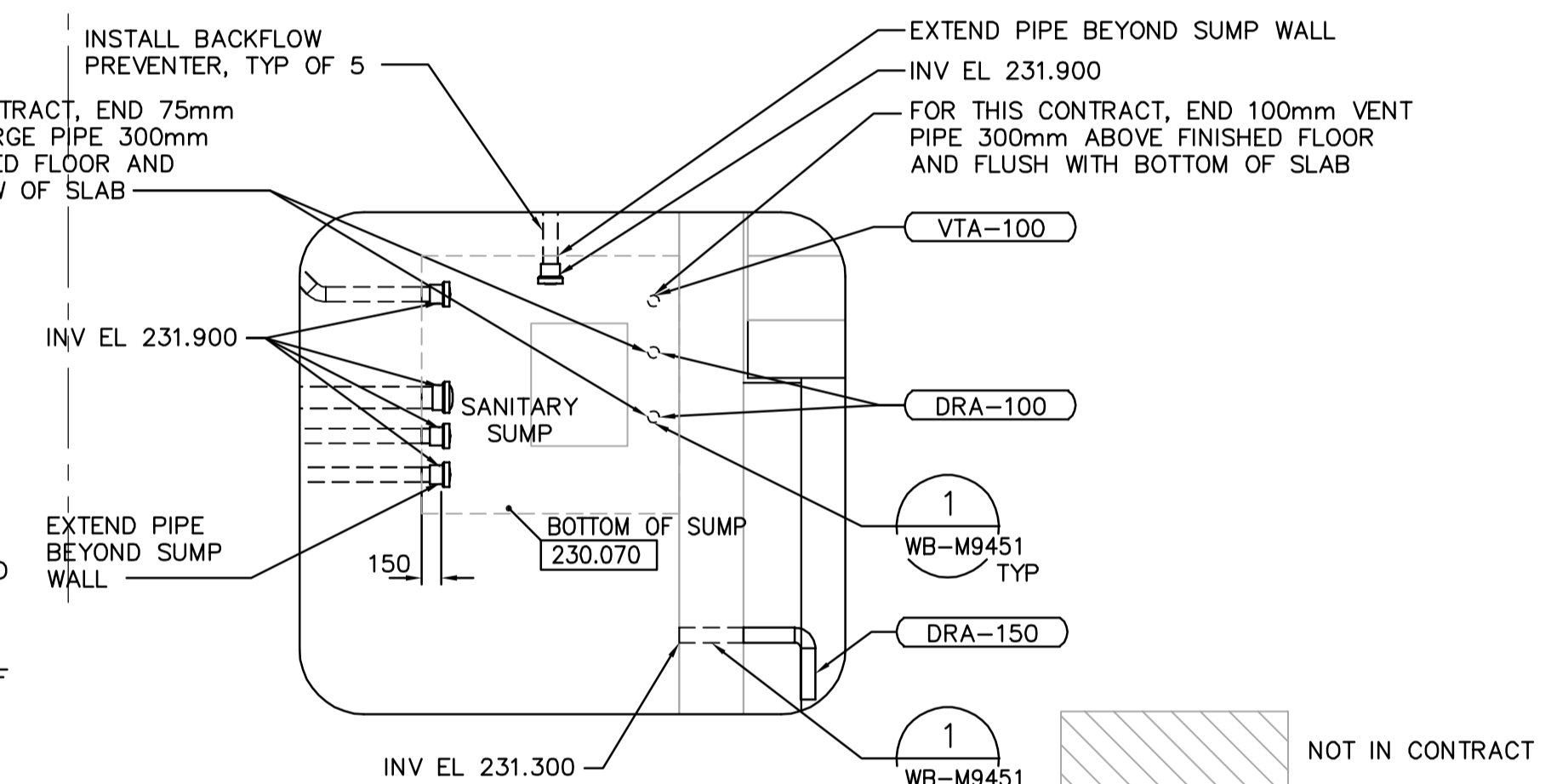
SOUTH SUMP DETAIL 1:50
